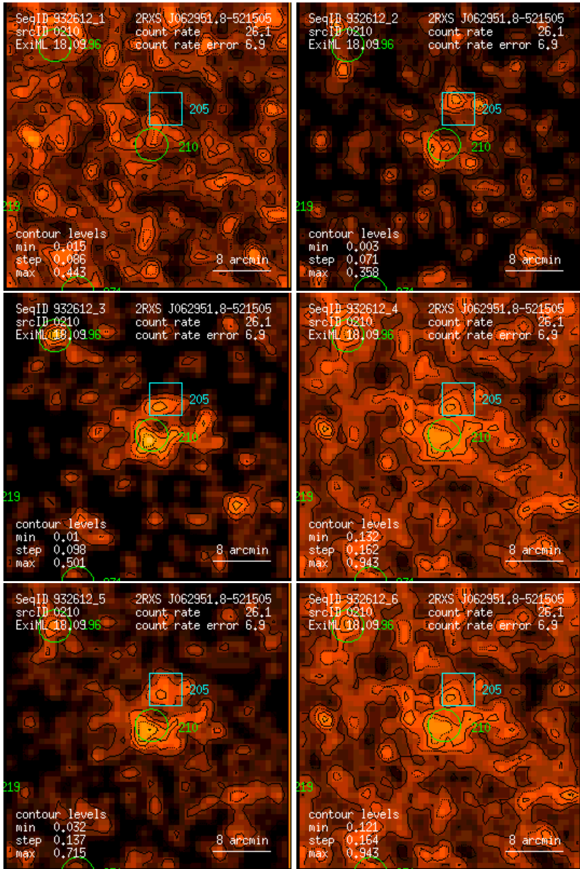
Figure 210: RASS 932612: detection 0210: band rate images, Gaussian filter: (1) PSPC channels 11 – 41, (2) 52 – 90, (3) 91 – 201, (4) 11 – 235, (5) 52 – 201, (6) 11 – 201. Broad band rates in counts/ks. Band rate contour levels in counts/ks/arcmin 2 .
