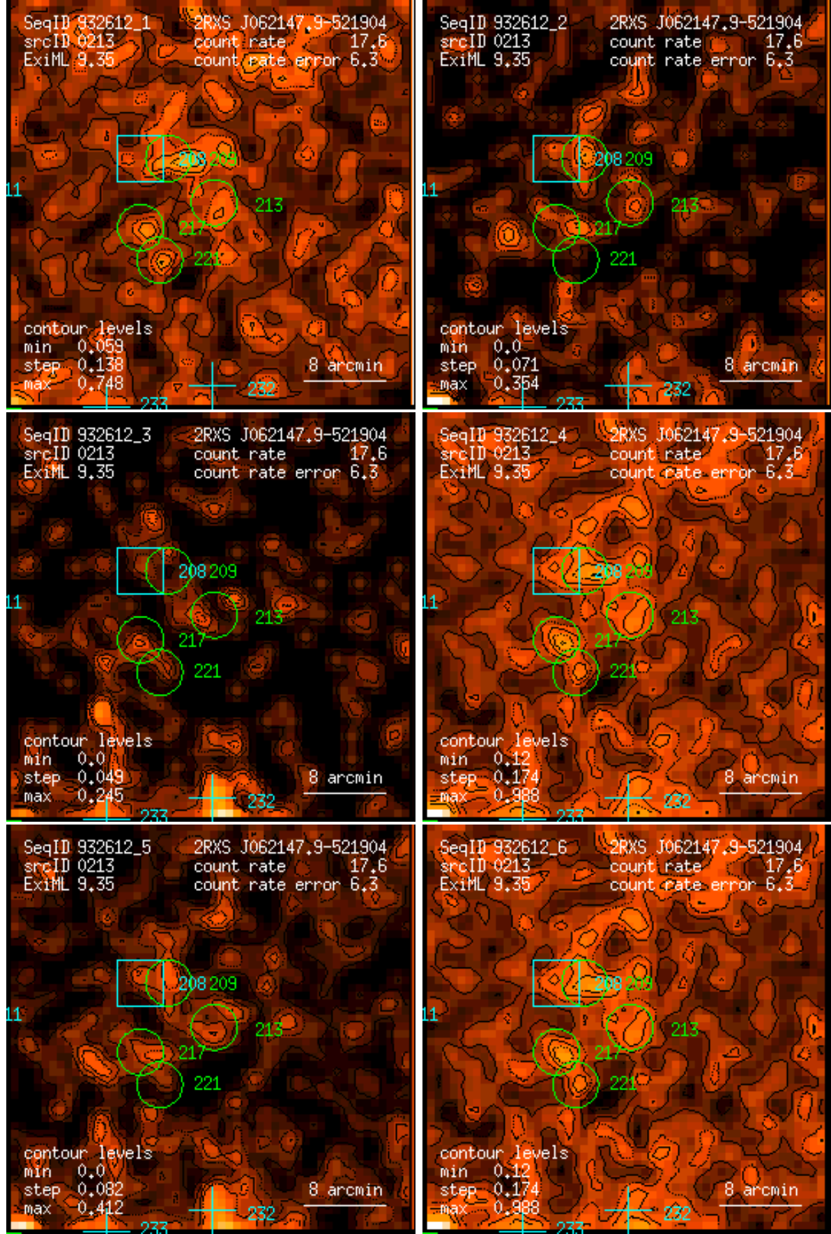
Figure 213: RASS 932612: detection 0213: band rate images, Gaussian filter: (1) PSPC channels 11 – 41, (2) 52 – 90, (3) 91 – 201, (4) 11 – 235, (5) 52 – 201, (6) 11 – 201. Broad band rates in counts/ks. Band rate contour levels in counts/ks/arcmin 2 .
