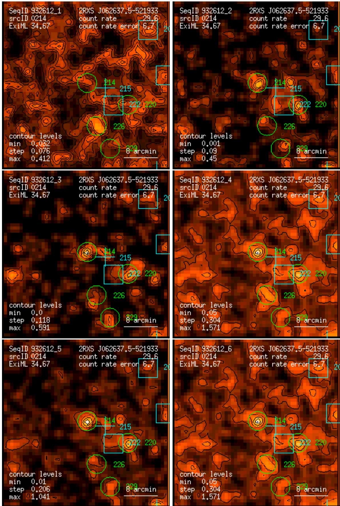
Figure 214: RASS 932612: detection 0214: band rate images, Gaussian filter: (1) PSPC channels 11 – 41, (2) 52 – 90, (3) 91 – 201, (4) 11 – 235, (5) 52 – 201, (6) 11 – 201. Broad band rates in counts/ks. Band rate contour levels in counts/ks/arcmin 2 .
