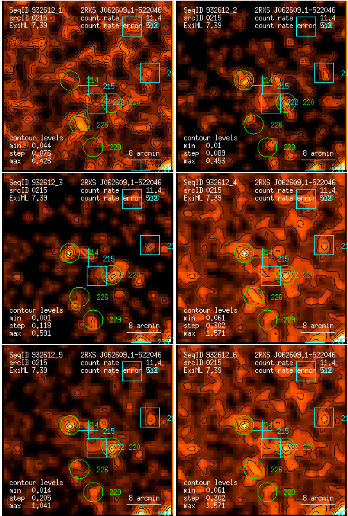
Figure 215: RASS 932612: detection 0215: band rate images, Gaussian filter: (1) PSPC channels 11 – 41, (2) 52 – 90, (3) 91 – 201, (4) 11 – 235, (5) 52 – 201, (6) 11 – 201. Broad band rates in counts/ks. Band rate contour levels in counts/ks/arcmin 2 .
