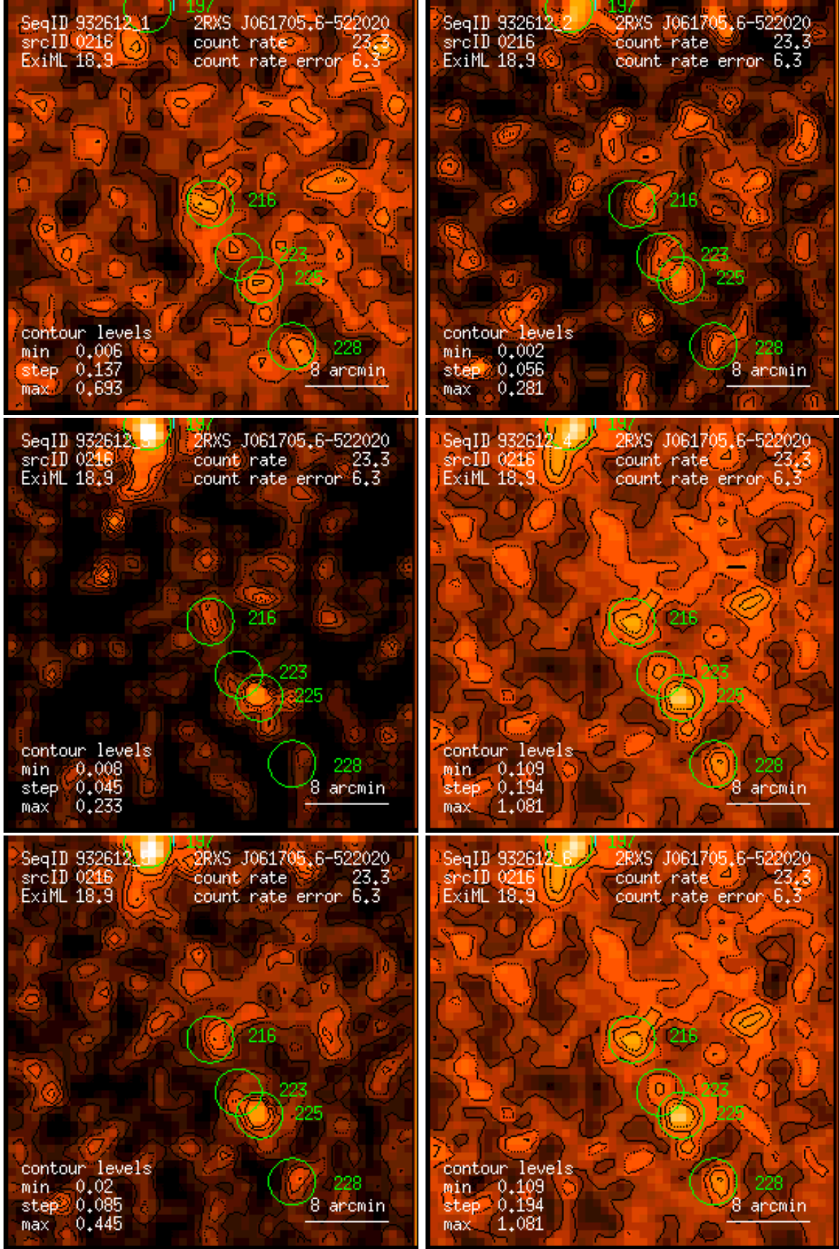
Figure 216: RASS 932612: detection 0216: band rate images, Gaussian filter: (1) PSPC channels 11 – 41, (2) 52 – 90, (3) 91 – 201, (4) 11 – 235, (5) 52 – 201, (6) 11 – 201. Broad band rates in counts/ks. Band rate contour levels in counts/ks/arcmin 2 .
