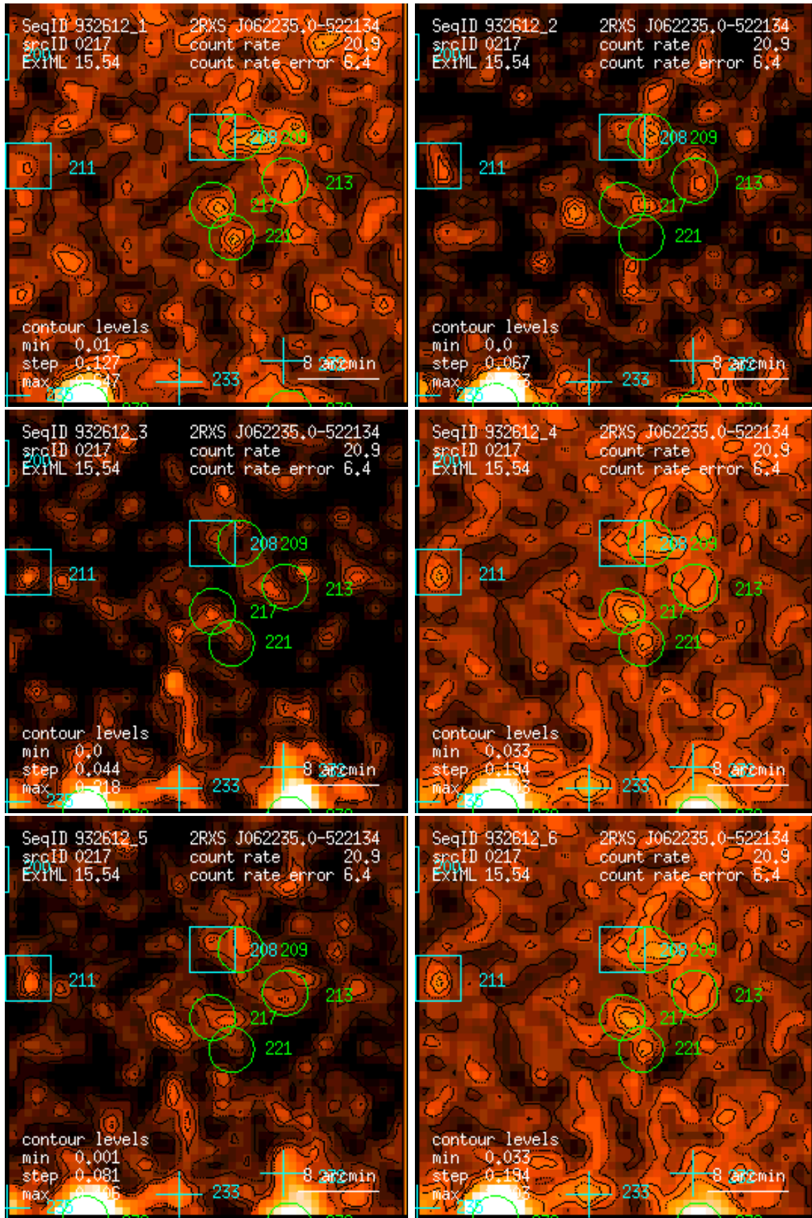
Figure 217: RASS 932612: detection 0217: band rate images, Gaussian filter: (1) PSPC channels 11 – 41, (2) 52 – 90, (3) 91 – 201, (4) 11 – 235, (5) 52 – 201, (6) 11 – 201. Broad band rates in counts/ks. Band rate contour levels in counts/ks/arcmin 2 .
