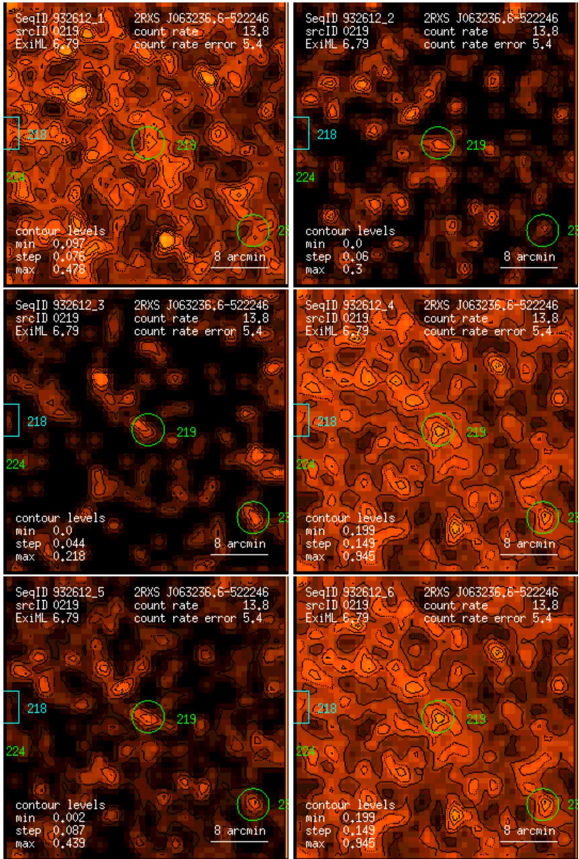
Figure 219: RASS 932612: detection 0219: band rate images, Gaussian filter: (1) PSPC channels 11 – 41, (2) 52 – 90, (3) 91 – 201, (4) 11 – 235, (5) 52 – 201, (6) 11 – 201. Broad band rates in counts/ks. Band rate contour levels in counts/ks/arcmin 2 .
