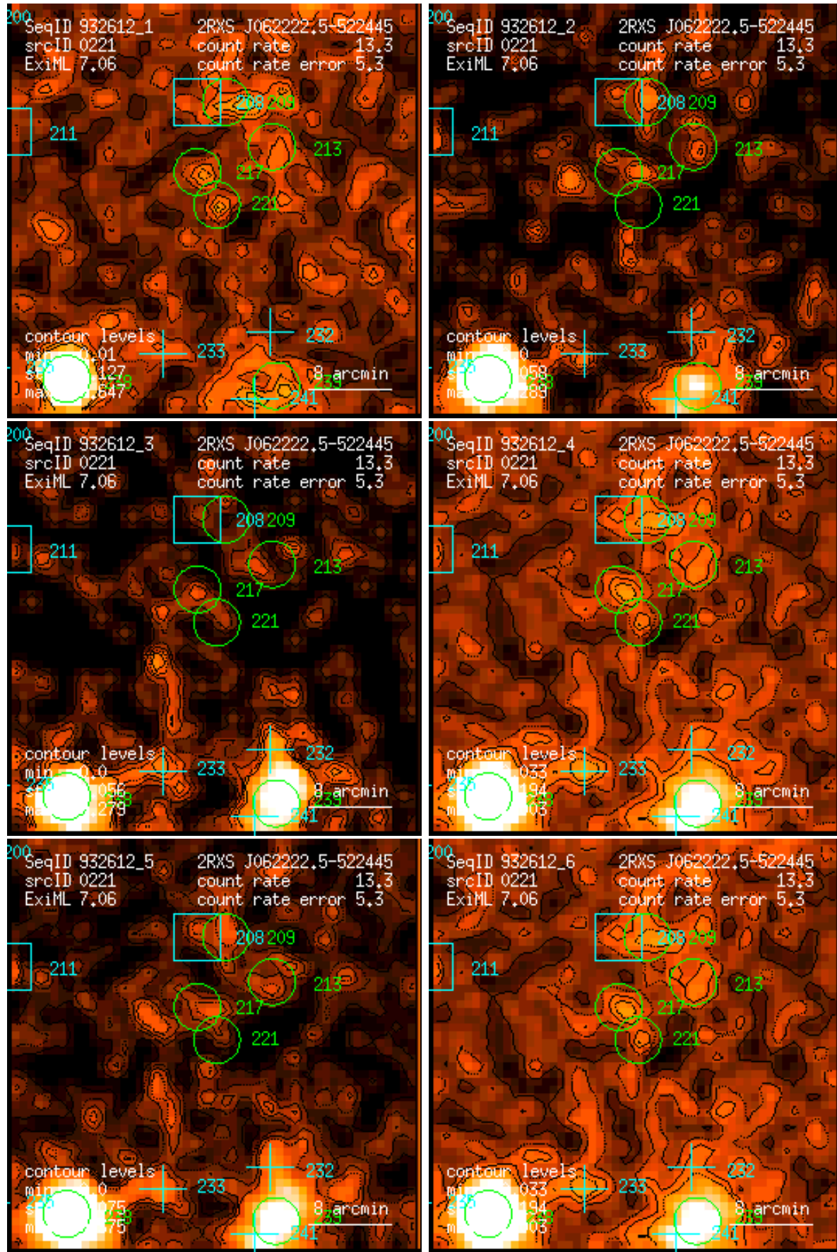
Figure 221: RASS 932612: detection 0221: band rate images, Gaussian filter: (1) PSPC channels 11 – 41, (2) 52 – 90, (3) 91 – 201, (4) 11 – 235, (5) 52 – 201, (6) 11 – 201. Broad band rates in counts/ks. Band rate contour levels in counts/ks/arcmin 2 .
