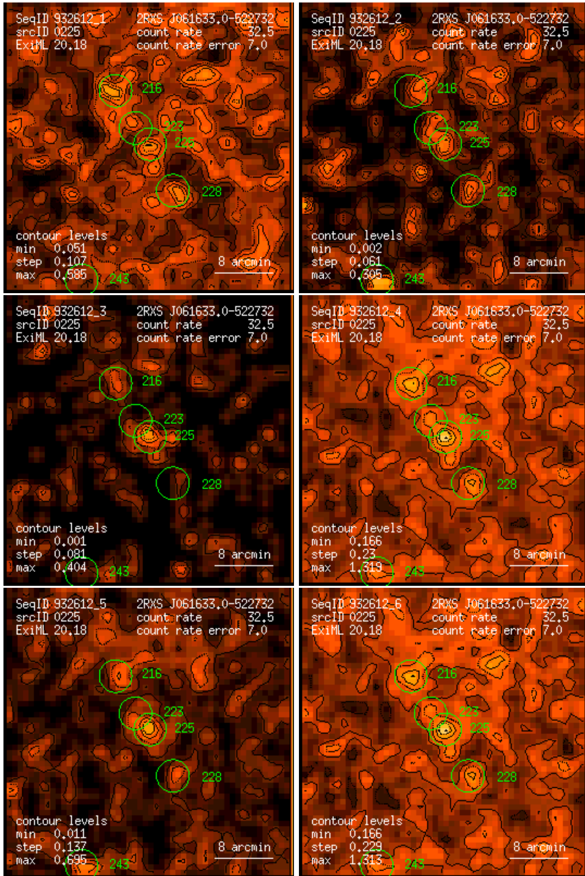
Figure 225: RASS 932612: detection 0225: band rate images, Gaussian filter: (1) PSPC channels 11 – 41, (2) 52 – 90, (3) 91 – 201, (4) 11 – 235, (5) 52 – 201, (6) 11 – 201. Broad band rates in counts/ks. Band rate contour levels in counts/ks/arcmin 2 .
