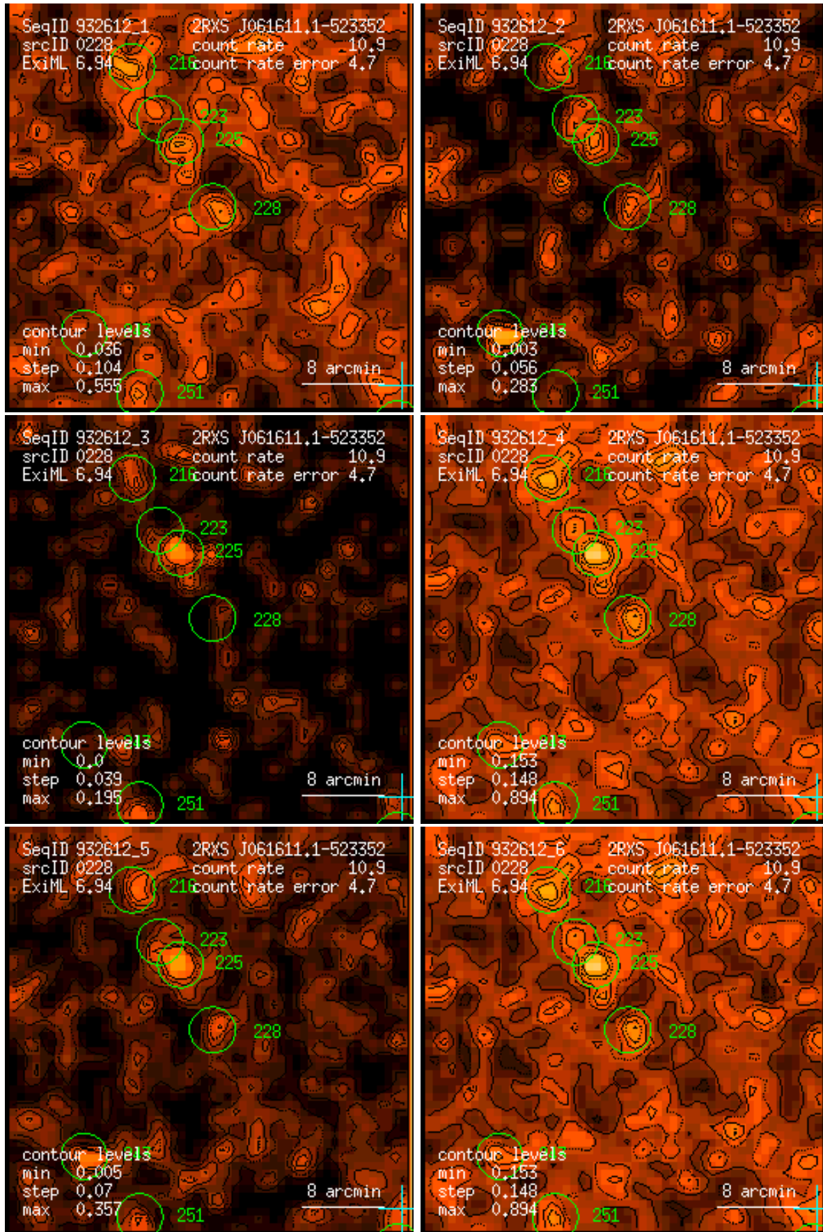
Figure 228: RASS 932612: detection 0228: band rate images, Gaussian filter: (1) PSPPC channels 11 – 41, (2) 52 – 90, (3) 91 – 201, (4) 11 – 235, (5) 52 – 201, (6) 11 – 201. Broad band rates in counts/ks. Band rate contour levels in counts/ks/arcmin 2 .
