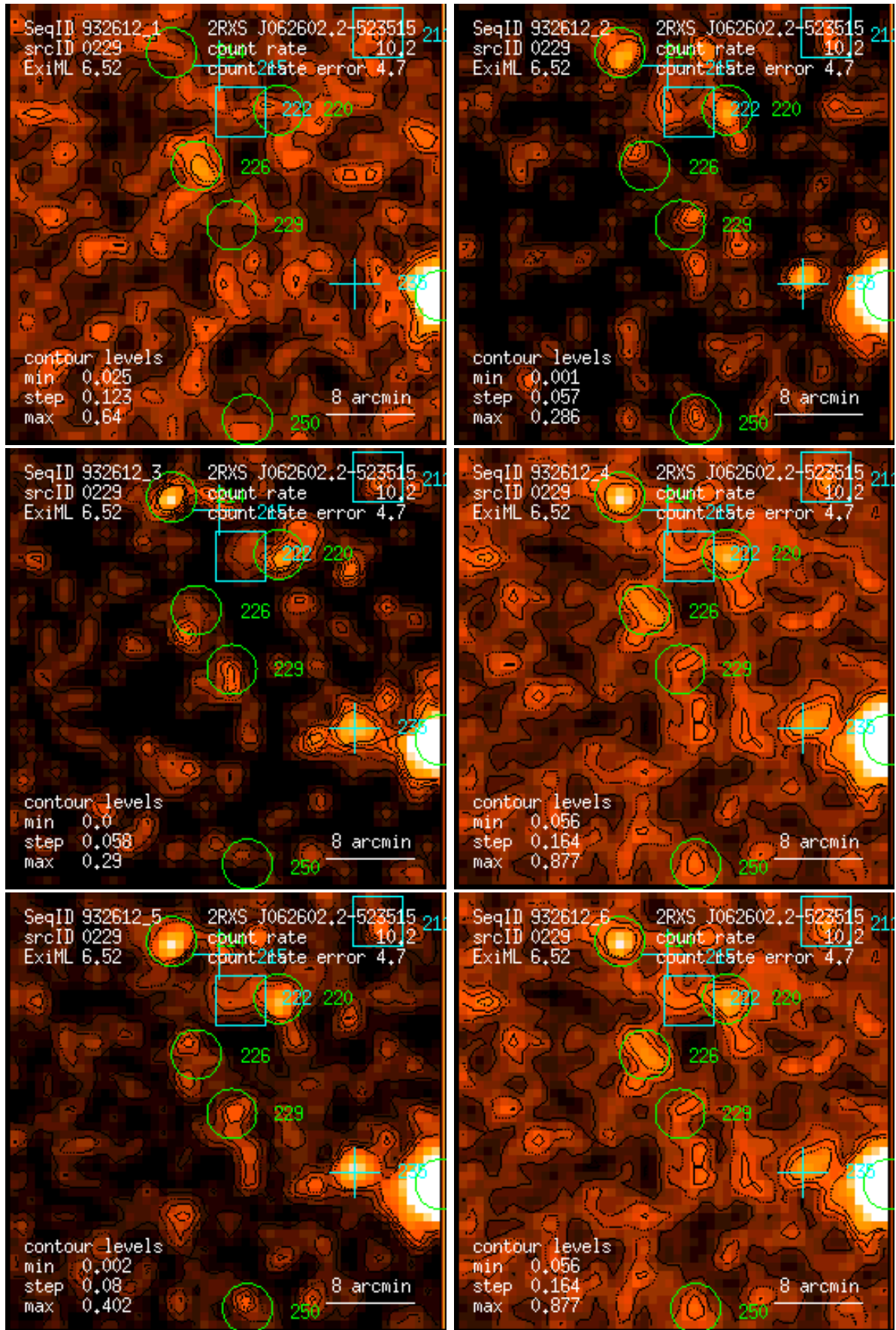
Figure 229: RASS 932612: detection 0229: band rate images, Gaussian filter: (1) PSPC channels 11 – 41, (2) 52 – 90, (3) 91 – 201, (4) 11 – 235, (5) 52 – 201, (6) 11 – 201. Broad band rates in counts/ks. Band rate contour levels in counts/ks/arcmin 2 .
