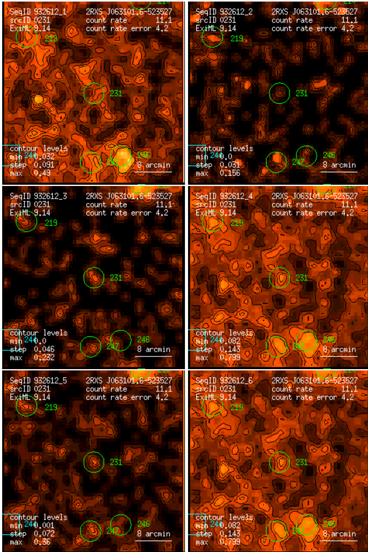
Figure 231: RASS 932612: detection 0231: band rate images, Gaussian filter: (1) PSPC channels 11 – 41, (2) 52 – 90, (3) 91 – 201, (4) 11 – 235, (5) 52 – 201, (6) 11 – 201. Broad band rates in counts/ks. Band rate contour levels in counts/ks/arcmin 2 .
