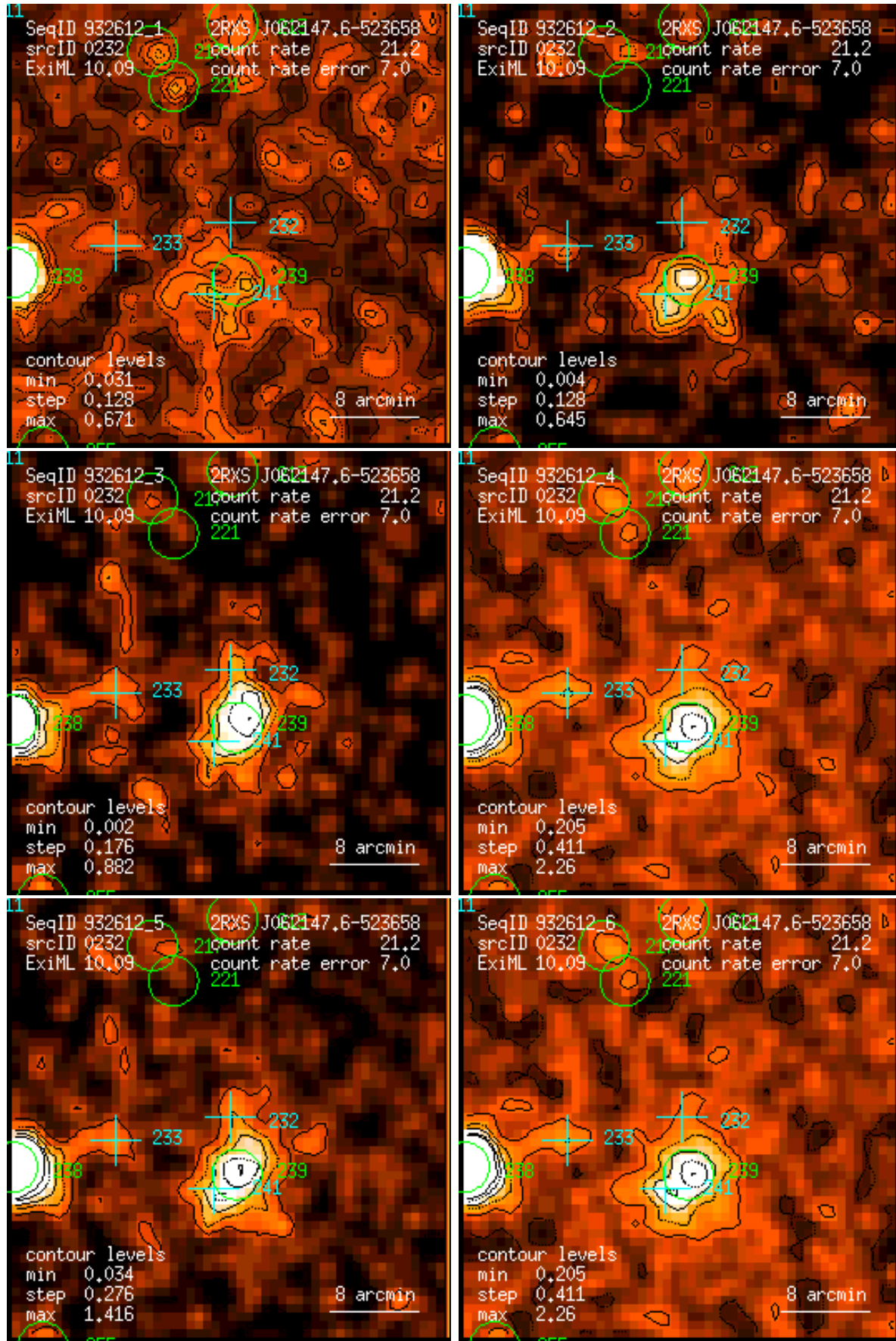
Figure 232: RASS 932612: detection 0232: band rate images, Gaussian filter: (1) PSPC channels 11 – 41, (2) 52 – 90, (3) 91 – 201, (4) 11 – 235, (5) 52 – 201, (6) 11 – 201. Broad band rates in counts/ks. Band rate contour levels in counts/ks/arcmin 2 .
