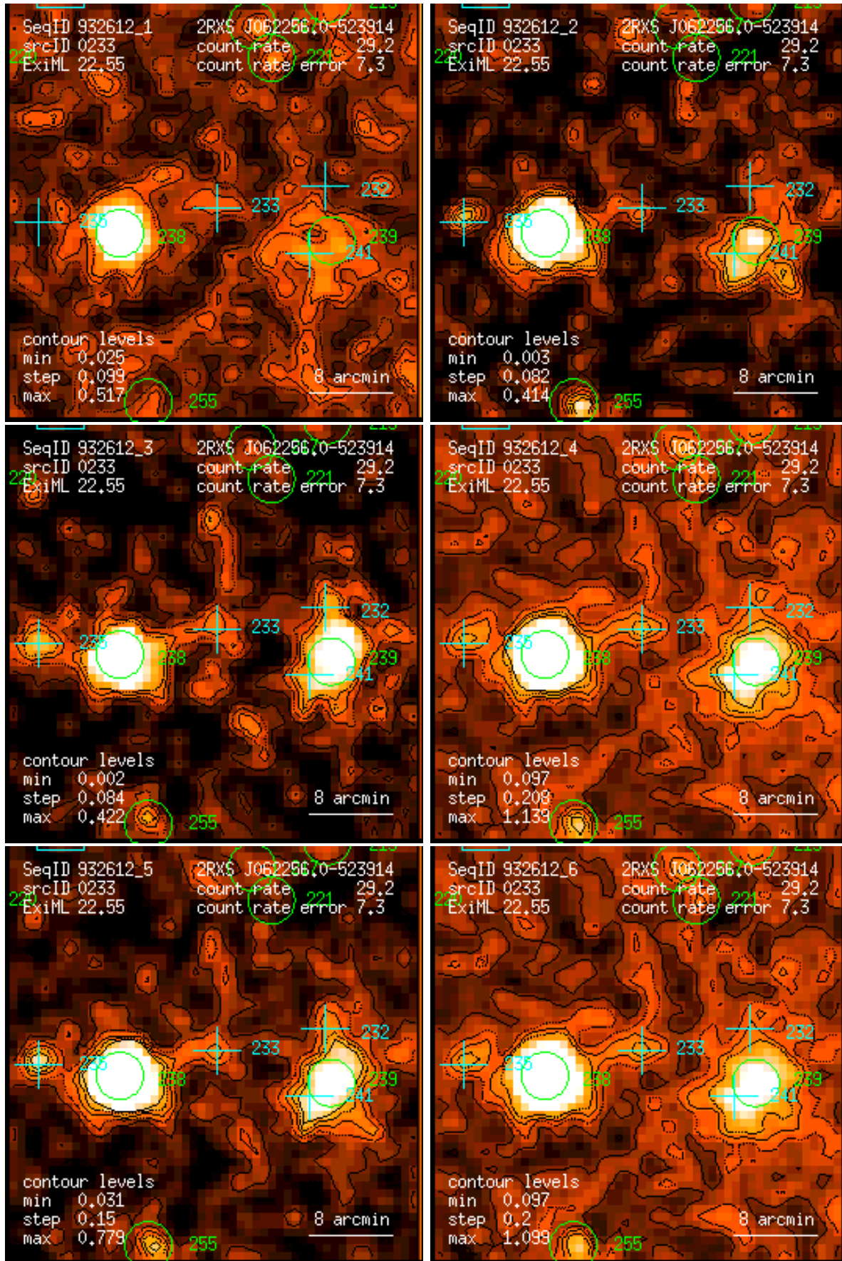
Figure 233: RASS 932612: detection 0233: band rate images, Gaussian filter: (1) PSPC channels 11 – 41, (2) 52 – 90, (3) 91 – 201, (4) 11 – 235, (5) 52 – 201, (6) 11 – 201. Broad band rates in counts/ks. Band rate contour levels in counts/ks/arcmin 2 .
