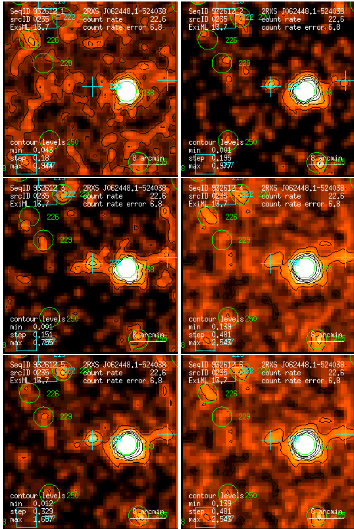
Figure 235: RASS 932612: detection 0235: band rate images, Gaussian filter: (1) PSPC channels 11 – 41, (2) 52 – 90, (3) 91 – 201, (4) 11 – 235, (5) 52 – 201, (6) 11 – 201. Broad band rates in counts/ks. Band rate contour levels in counts/ks/arcmin 2 .
