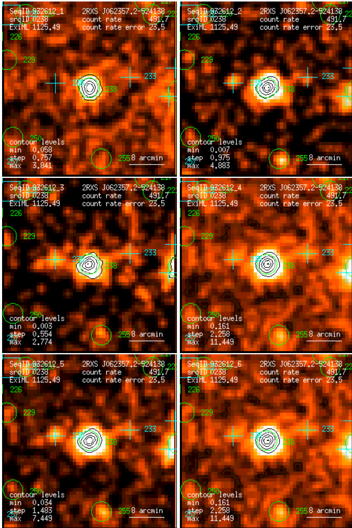
Figure 238: RASS 932612: detection 0238: band rate images, Gaussian filter: (1) PSPC channels 11 – 41, (2) 52 – 90, (3) 91 – 201, (4) 11 – 235, (5) 52 – 201, (6) 11 – 201. Broad band rates in counts/ks. Band rate contour levels in counts/ks/arcmin 2 .
