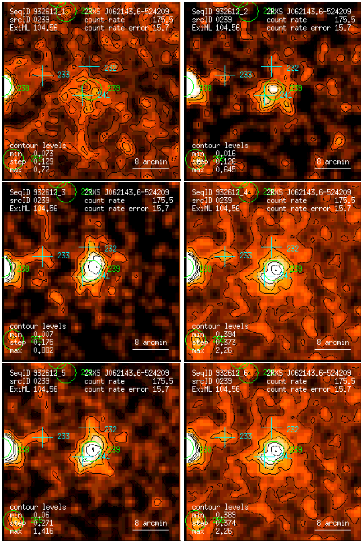
Figure 239: RASS 932612: detection 0239: band rate images, Gaussian filter: (1) PSPC channels 11 – 41, (2) 52 – 90, (3) 91 – 201, (4) 11 – 235, (5) 52 – 201, (6) 11 – 201. Broad band rates in counts/ks. Band rate contour levels in counts/ks/arcmin 2 .
