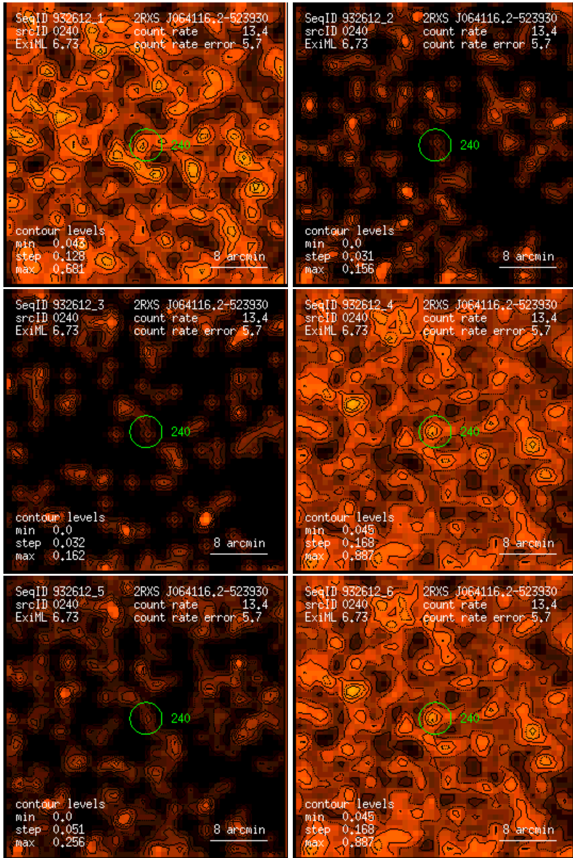
Figure 240: RASS 932612: detection 0240: band rate images, Gaussian filter: (1) PSPC channels 11 – 41, (2) 52 – 90, (3) 91 – 201, (4) 11 – 235, (5) 52 – 201, (6) 11 – 201. Broad band rates in counts/ks. Band rate contour levels in counts/ks/arcmin 2 .
