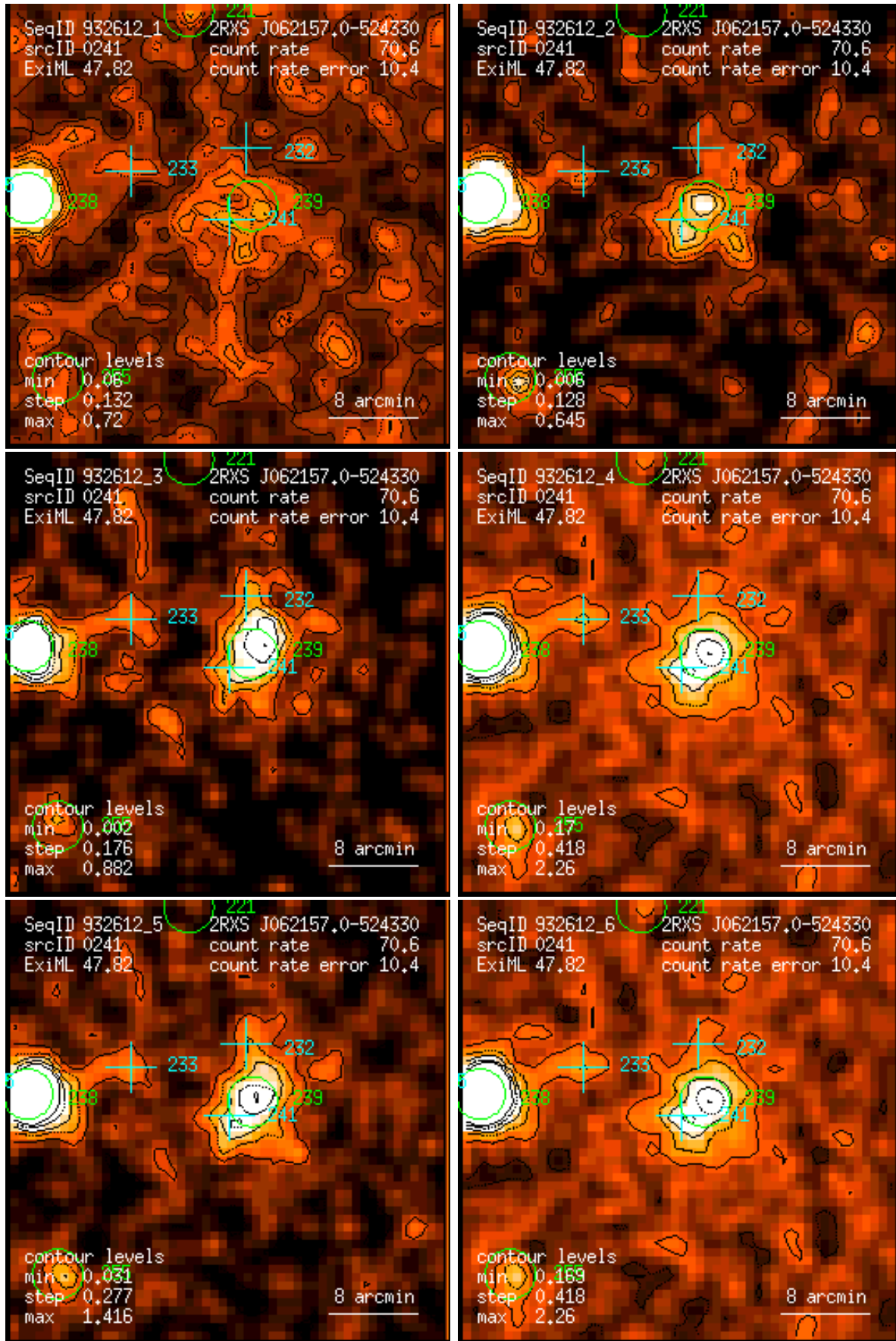
Figure 241: RASS 932612: detection 0241: band rate images, Gaussian filter: (1) PSPC channels 11 – 41, (2) 52 – 90, (3) 91 – 201, (4) 11 – 235, (5) 52 – 201, (6) 11 – 201. Broad band rates in counts/ks. Band rate contour levels in counts/ks/arcmin 2 .
