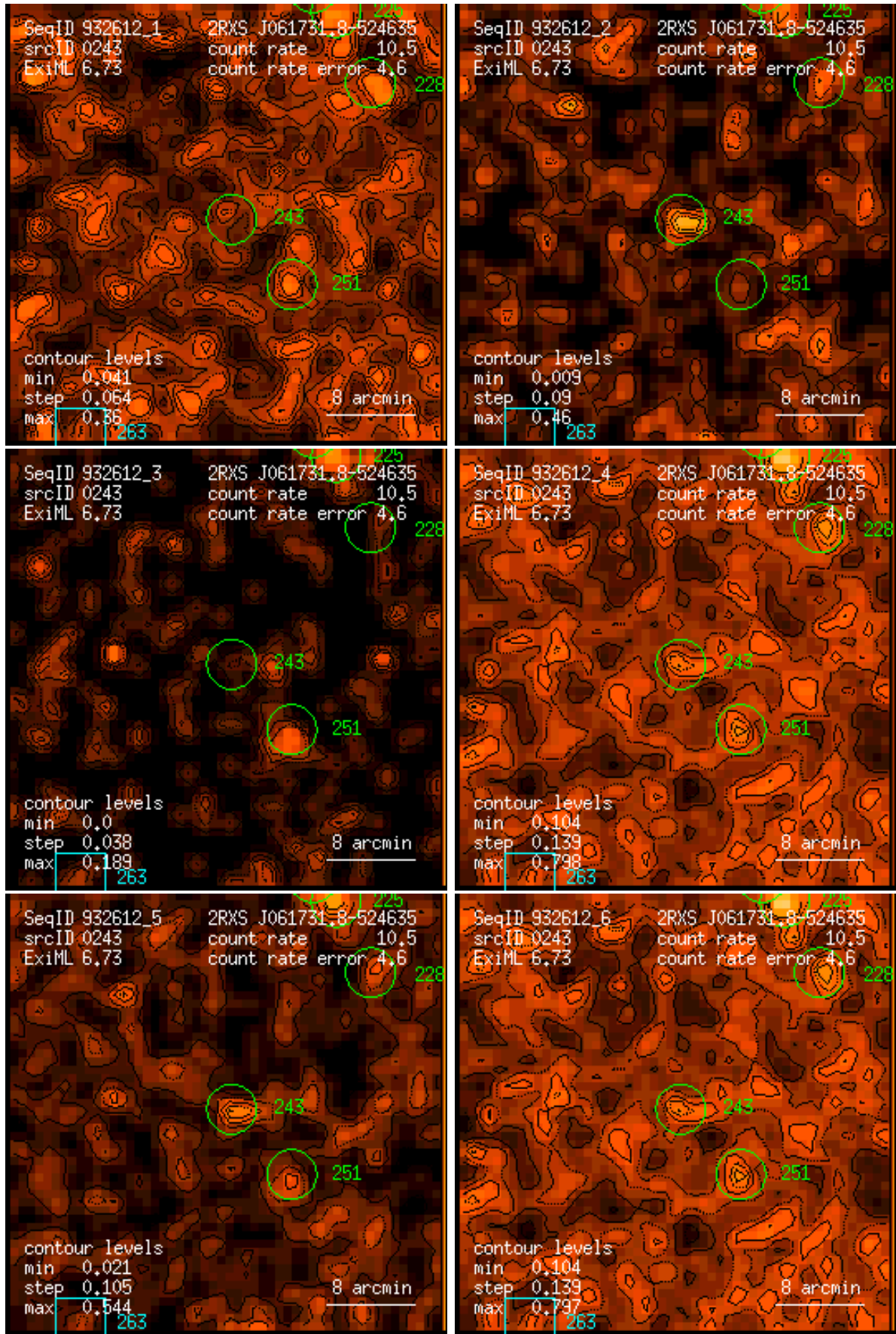
Figure 243: RASS 932612: detection 0243: band rate images, Gaussian filter: (1) PSPC channels 11 – 41, (2) 52 – 90, (3) 91 – 201, (4) 11 – 235, (5) 52 – 201, (6) 11 – 201. Broad band rates in counts/ks. Band rate contour levels in counts/ks/arcmin 2 .
