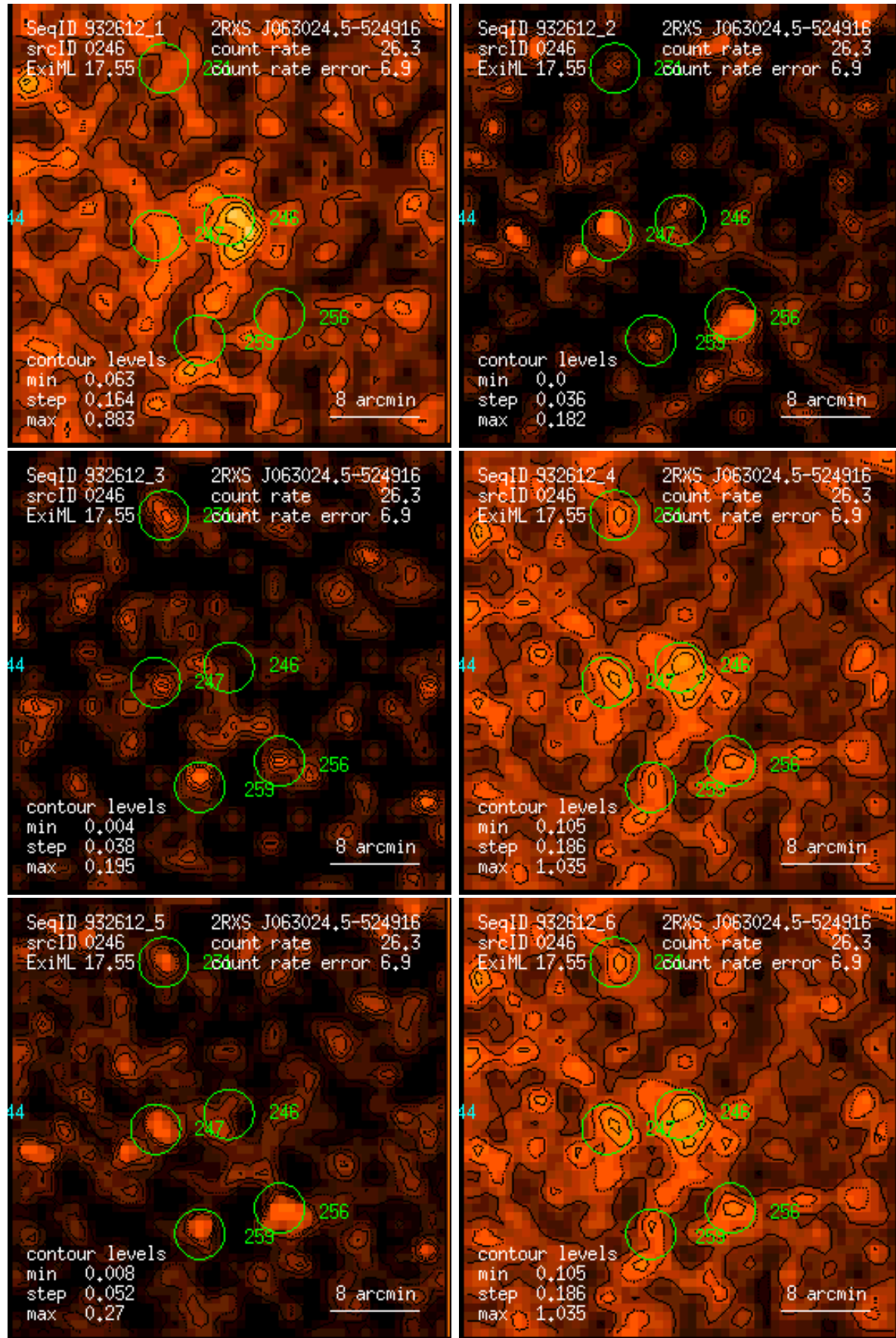
Figure 246: RASS 932612: detection 0246: band rate images, Gaussian filter: (1) PSPC channels 11 – 41, (2) 52 – 90, (3) 91 – 201, (4) 11 – 235, (5) 52 – 201, (6) 11 – 201. Broad band rates in counts/ks. Band rate contour levels in counts/ks/arcmin 2 .
