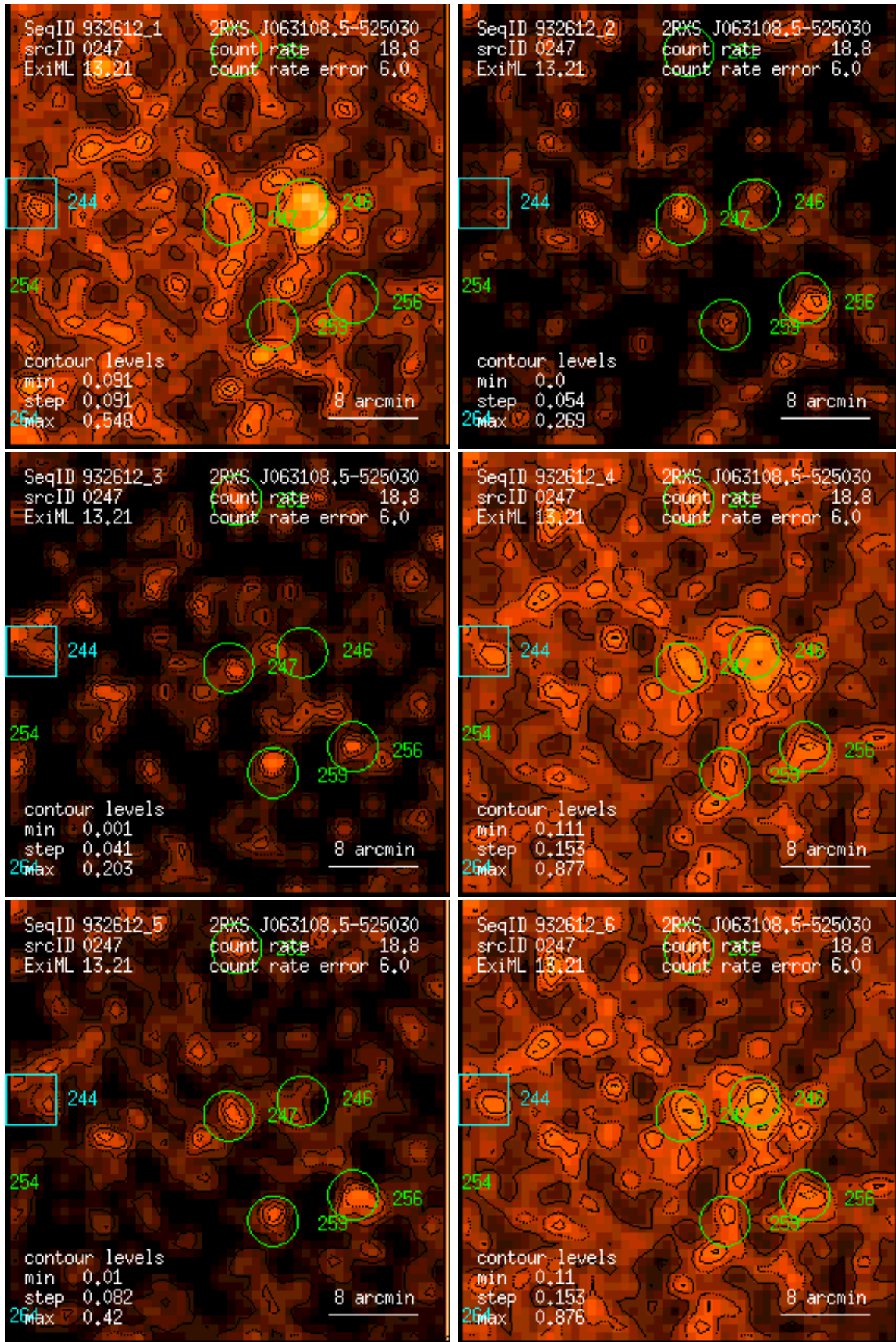
Figure 247: RASS 932612: detection 0247: band rate images, Gaussian filter: (1) PSPC channels 11 – 41, (2) 52 – 90, (3) 91 – 201, (4) 11 – 235, (5) 52 – 201, (6) 11 – 201. Broad band rates in counts/ks. Band rate contour levels in counts/ks/arcmin 2 .
