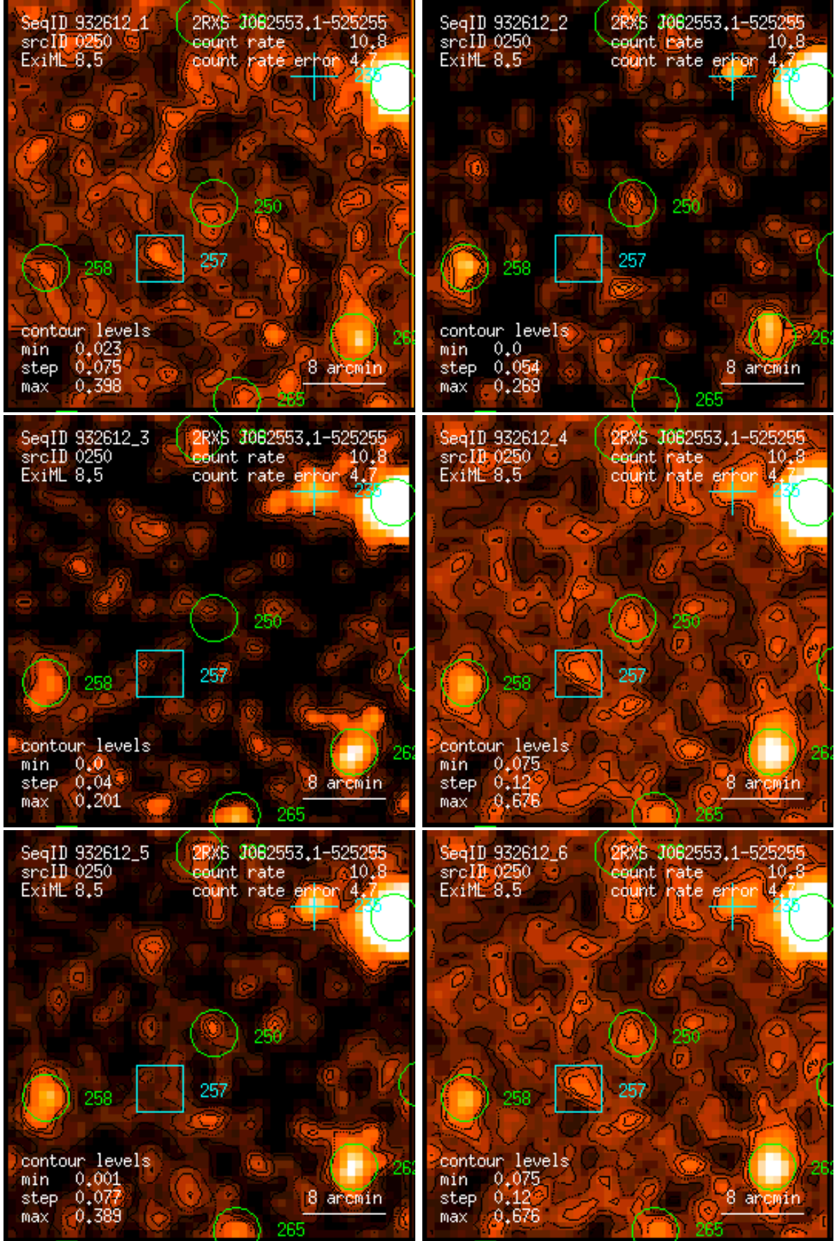
Figure 250: RASS 932612: detection 0250: band rate images, Gaussian filter: (1) PSPC channels 11 – 41, (2) 52 – 90, (3) 91 – 201, (4) 11 – 235, (5) 52 – 201, (6) 11 – 201. Broad band rates in counts/ks. Band rate contour levels in counts/ks/arcmin 2 .
