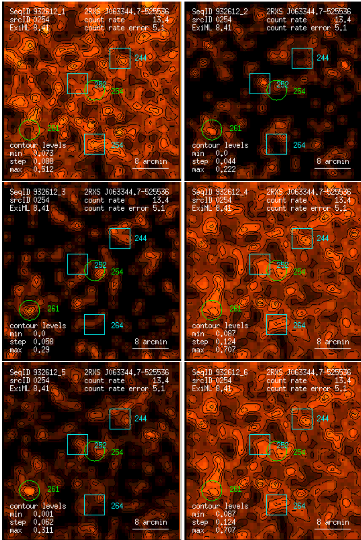
Figure 254: RASS 932612: detection 0254: band rate images, Gaussian filter: (1) PSPC channels 11 – 41, (2) 52 – 90, (3) 91 – 201, (4) 11 – 235, (5) 52 – 201, (6) 11 – 201. Broad band rates in counts/ks. Band rate contour levels in counts/ks/arcmin 2 .
