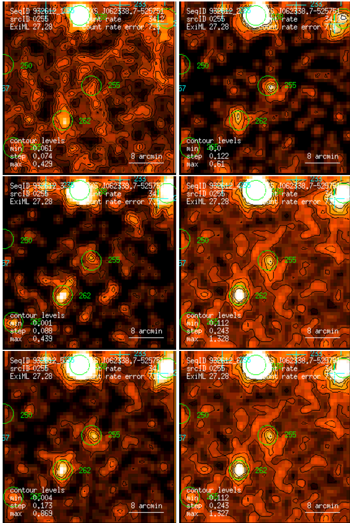
Figure 255: RASS 932612: detection 0255: band rate images, Gaussian filter: (1) PSPC channels 11 – 41, (2) 52 – 90, (3) 91 – 201, (4) 11 – 235, (5) 52 – 201, (6) 11 – 201. Broad band rates in counts/ks. Band rate contour levels in counts/ks/arcmin 2 .
