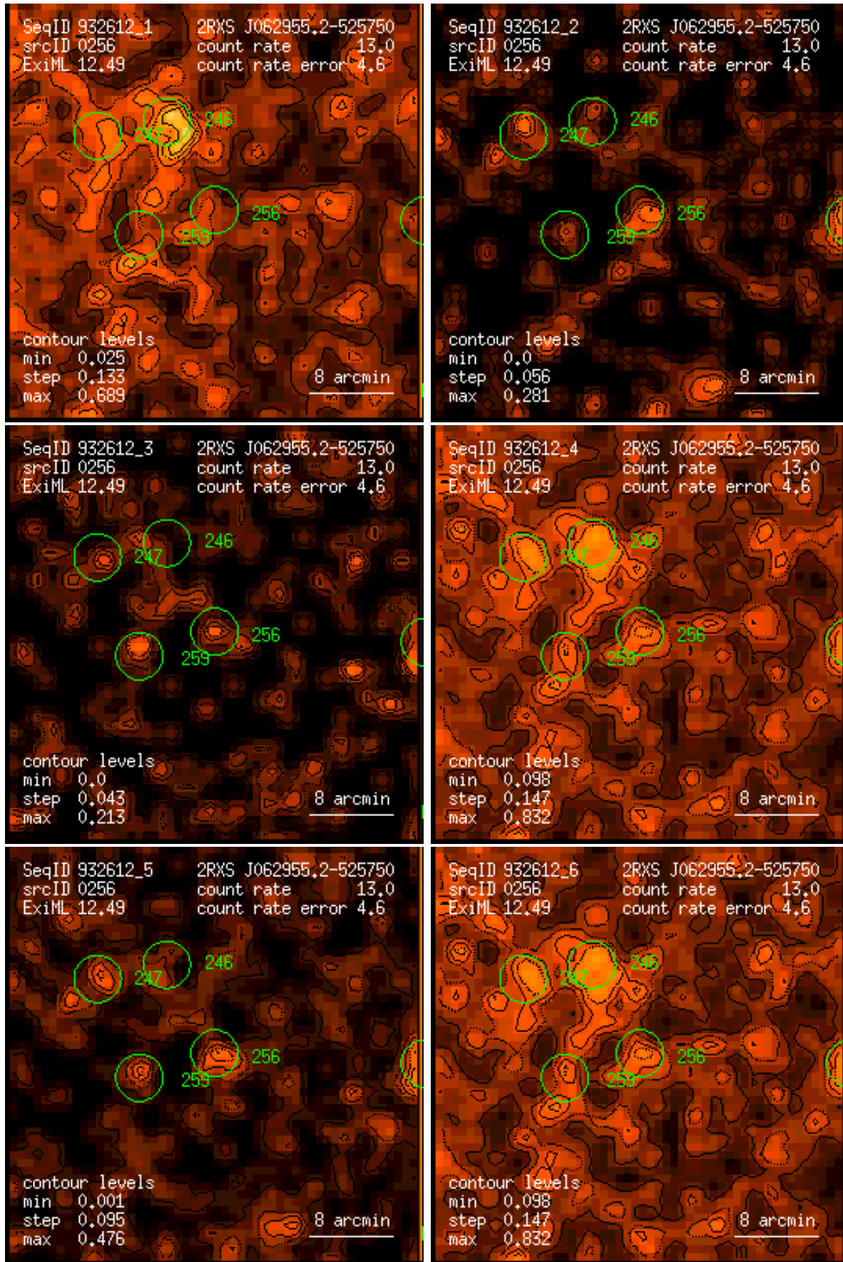
Figure 256: RASS 932612: detection 0256: band rate images, Gaussian filter: (1) PSPC channels 11 – 41, (2) 52 – 90, (3) 91 – 201, (4) 11 – 235, (5) 52 – 201, (6) 11 – 201. Broad band rates in counts/ks. Band rate contour levels in counts/ks/arcmin 2 .
