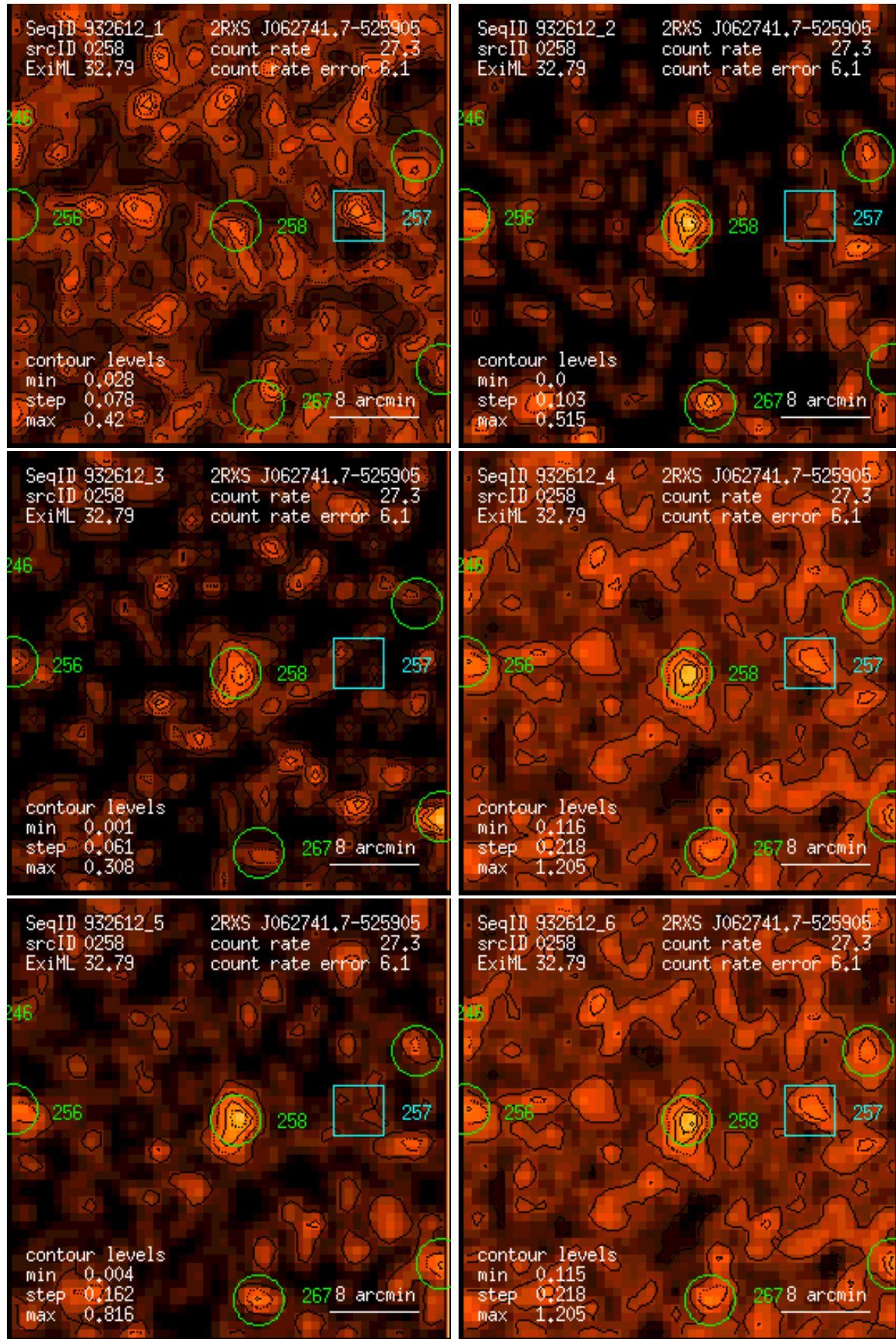
Figure 258: RASS 932612: detection 0258: band rate images, Gaussian filter: (1) PSPC channels 11 – 41, (2) 52 – 90, (3) 91 – 201, (4) 11 – 235, (5) 52 – 201, (6) 11 – 201. Broad band rates in counts/ks. Band rate contour levels in counts/ks/arcmin 2 .
