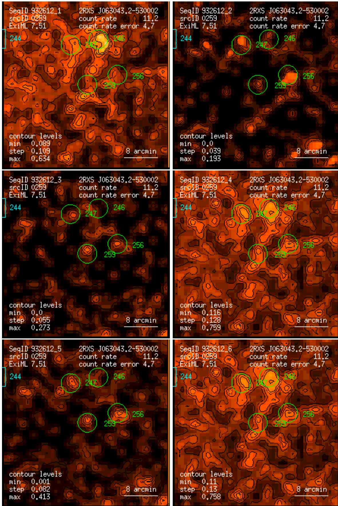
Figure 259: RASS 932612: detection 0259: band rate images, Gaussian filter: (1) PSPC channels 11 – 41, (2) 52 – 90, (3) 91 – 201, (4) 11 – 235, (5) 52 – 201, (6) 11 – 201. Broad band rates in counts/ks. Band rate contour levels in counts/ks/arcmin 2 .
