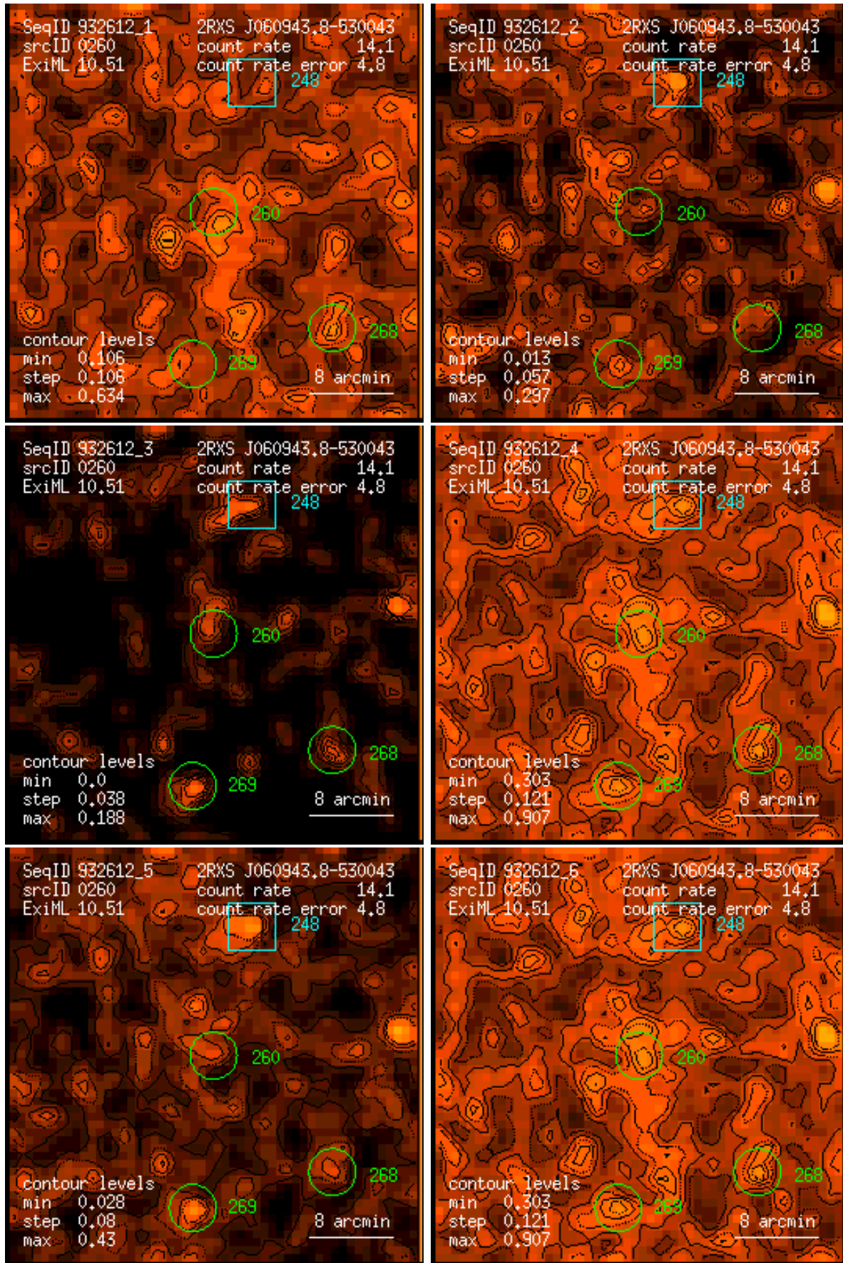
Figure 260: RASS 932612: detection 0260: band rate images, Gaussian filter: (1) PSPC channels 11 – 41, (2) 52 – 90, (3) 91 – 201, (4) 11 – 235, (5) 52 – 201, (6) 11 – 201. Broad band rates in counts/ks. Band rate contour levels in counts/ks/arcmin 2 .
