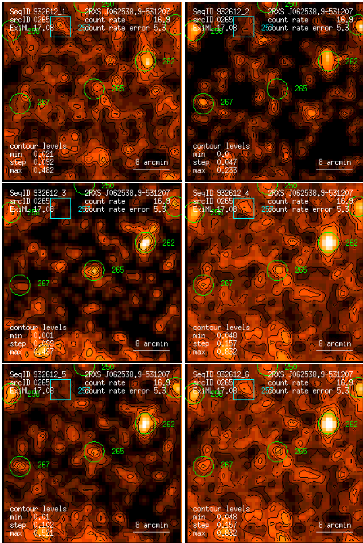
Figure 265: RASS 932612: detection 0265: band rate images, Gaussian filter: (1) PSPC channels 11 – 41, (2) 52 – 90, (3) 91 – 201, (4) 11 – 235, (5) 52 – 201, (6) 11 – 201. Broad band rates in counts/ks. Band rate contour levels in counts/ks/arcmin 2 .
