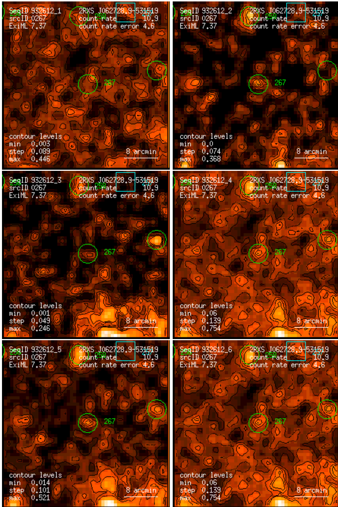
Figure 267: RASS 932612: detection 0267: band rate images, Gaussian filter: (1) PSPC channels 11 – 41, (2) 52 – 90, (3) 91 – 201, (4) 11 – 235, (5) 52 – 201, (6) 11 – 201. Broad band rates in counts/ks. Band rate contour levels in counts/ks/arcmin 2 .
