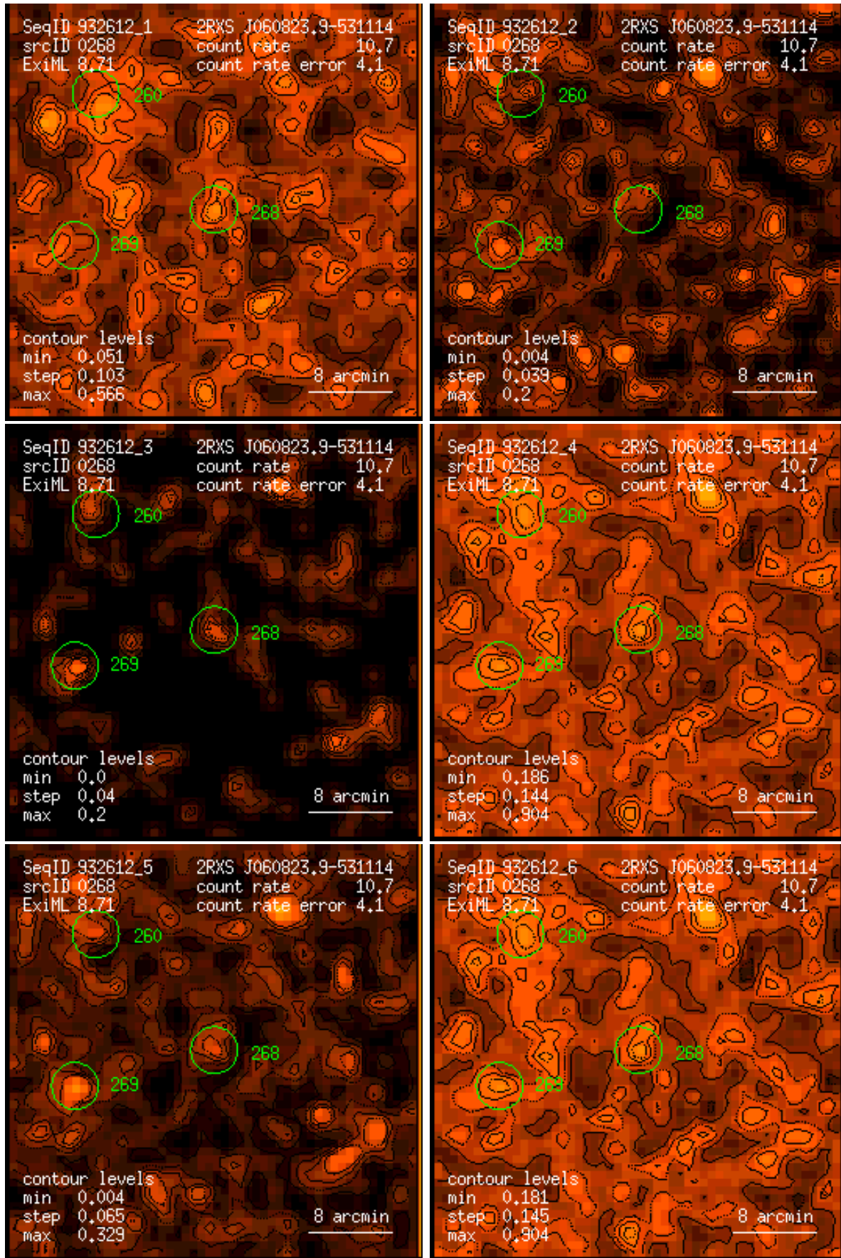
Figure 268: RASS 932612: detection 0268: band rate images, Gaussian filter: (1) PSPC channels 11 – 41, (2) 52 – 90, (3) 91 – 201, (4) 11 – 235, (5) 52 – 201, (6) 11 – 201. Broad band rates in counts/ks. Band rate contour levels in counts/ks/arcmin 2 .
