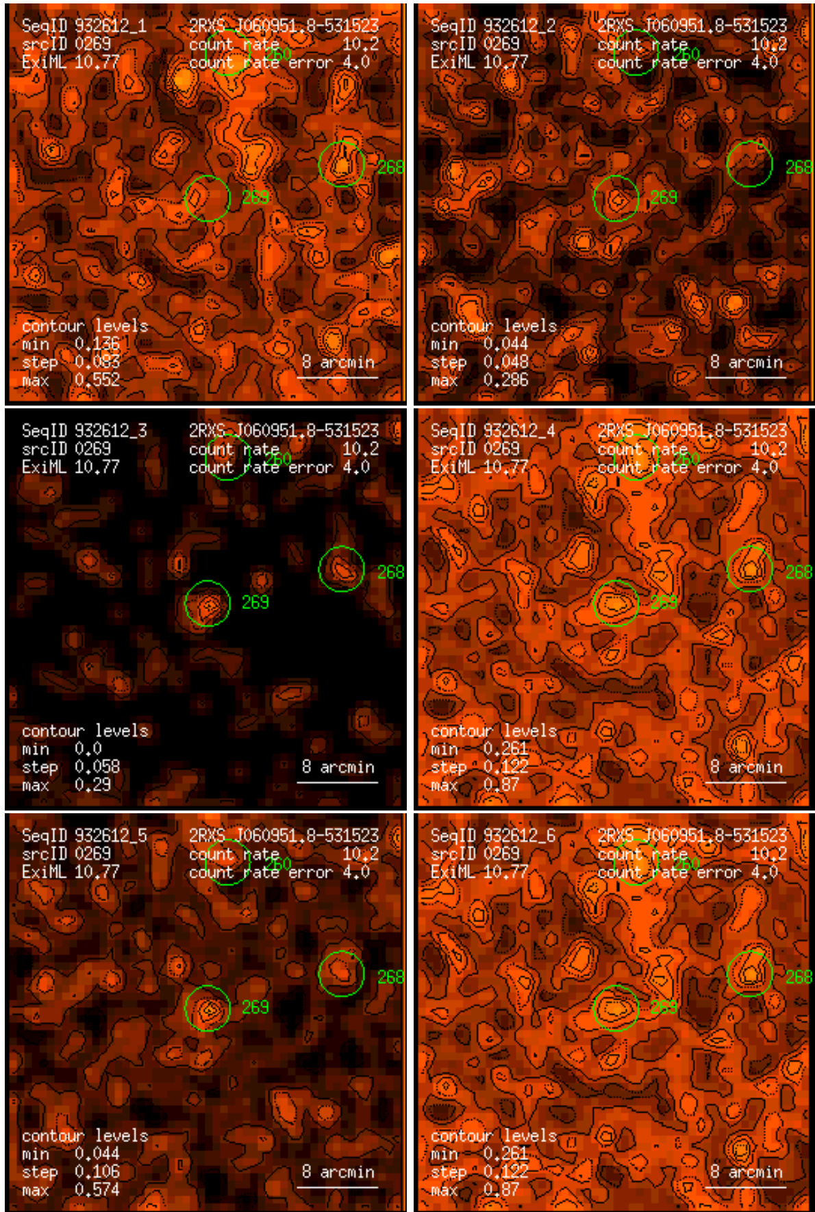
Figure 269: RASS 932612: detection 0269: band rate images, Gaussian filter: (1) PSPC channels 11 – 41, (2) 52 – 90, (3) 91 – 201, (4) 11 – 235, (5) 52 – 201, (6) 11 – 201. Broad band rates in counts/ks. Band rate contour levels in counts/ks/arcmin 2 .
