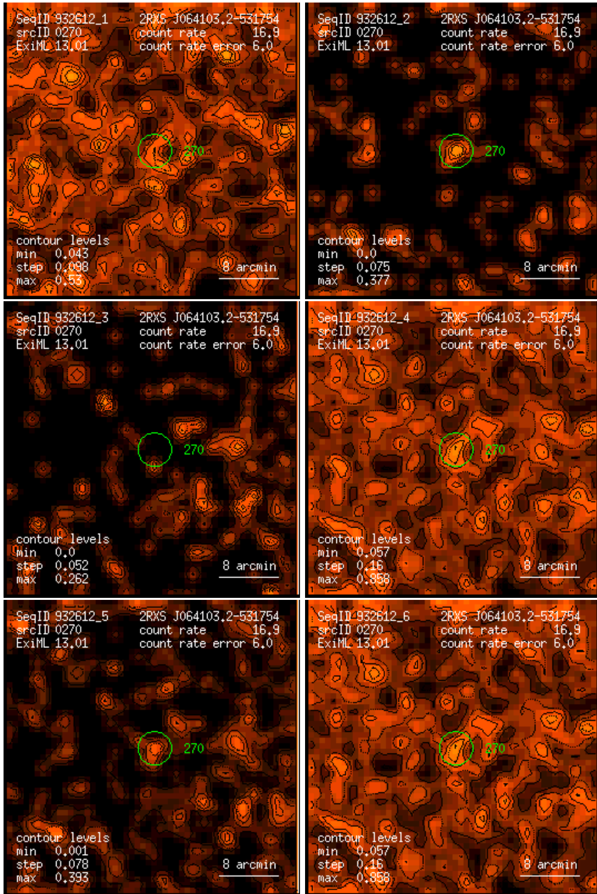
Figure 270: RASS 932612: detection 0270: band rate images, Gaussian filter: (1) PSPC channels 11 – 41, (2) 52 – 90, (3) 91 – 201, (4) 11 – 235, (5) 52 – 201, (6) 11 – 201. Broad band rates in counts/ks. Band rate contour levels in counts/ks/arcmin 2 .
