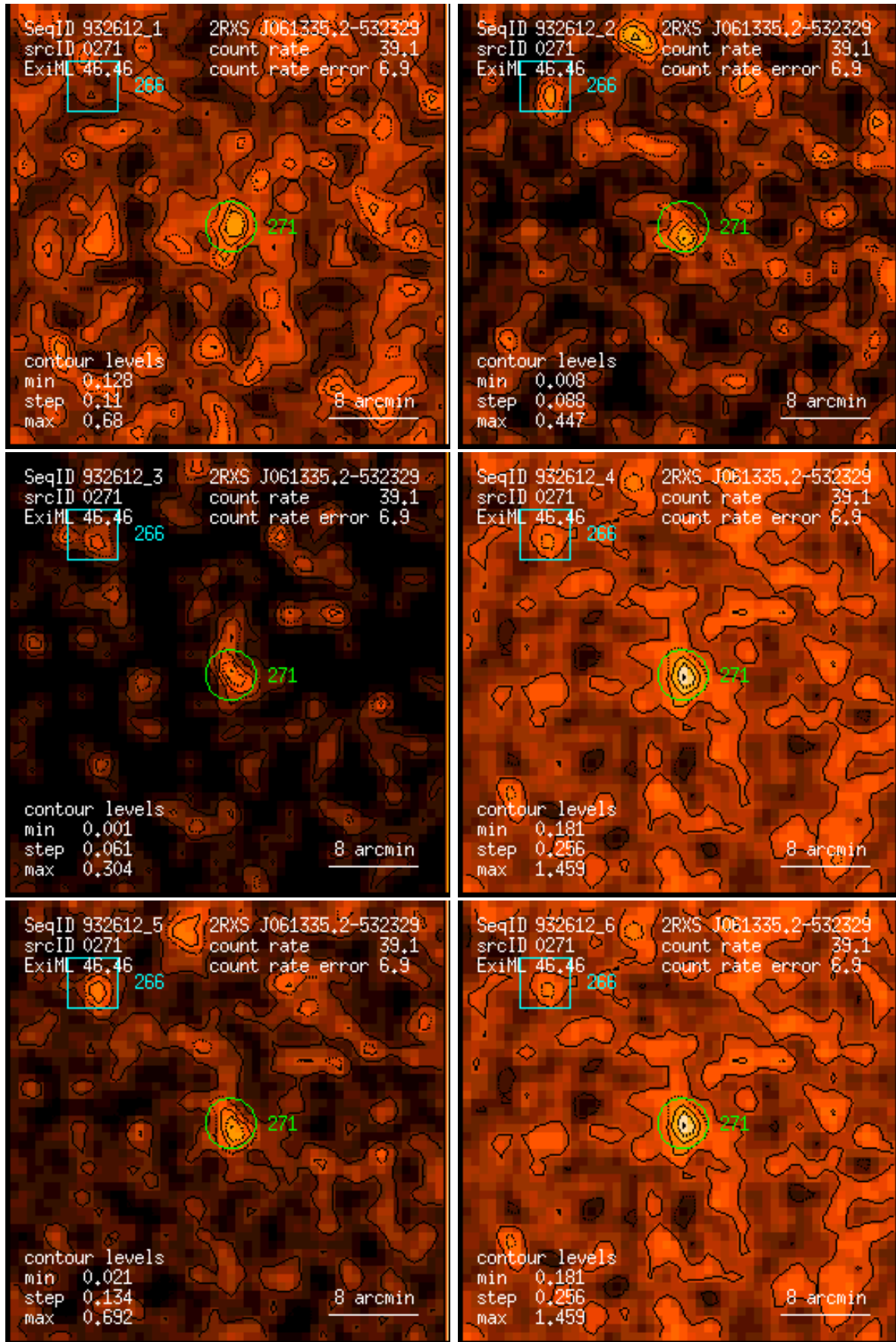
Figure 271: RASS 932612: detection 0271: band rate images, Gaussian filter: (1) PSPC channels 11 – 41, (2) 52 – 90, (3) 91 – 201, (4) 11 – 235, (5) 52 – 201, (6) 11 – 201. Broad band rates in counts/ks. Band rate contour levels in counts/ks/arcmin 2 .
