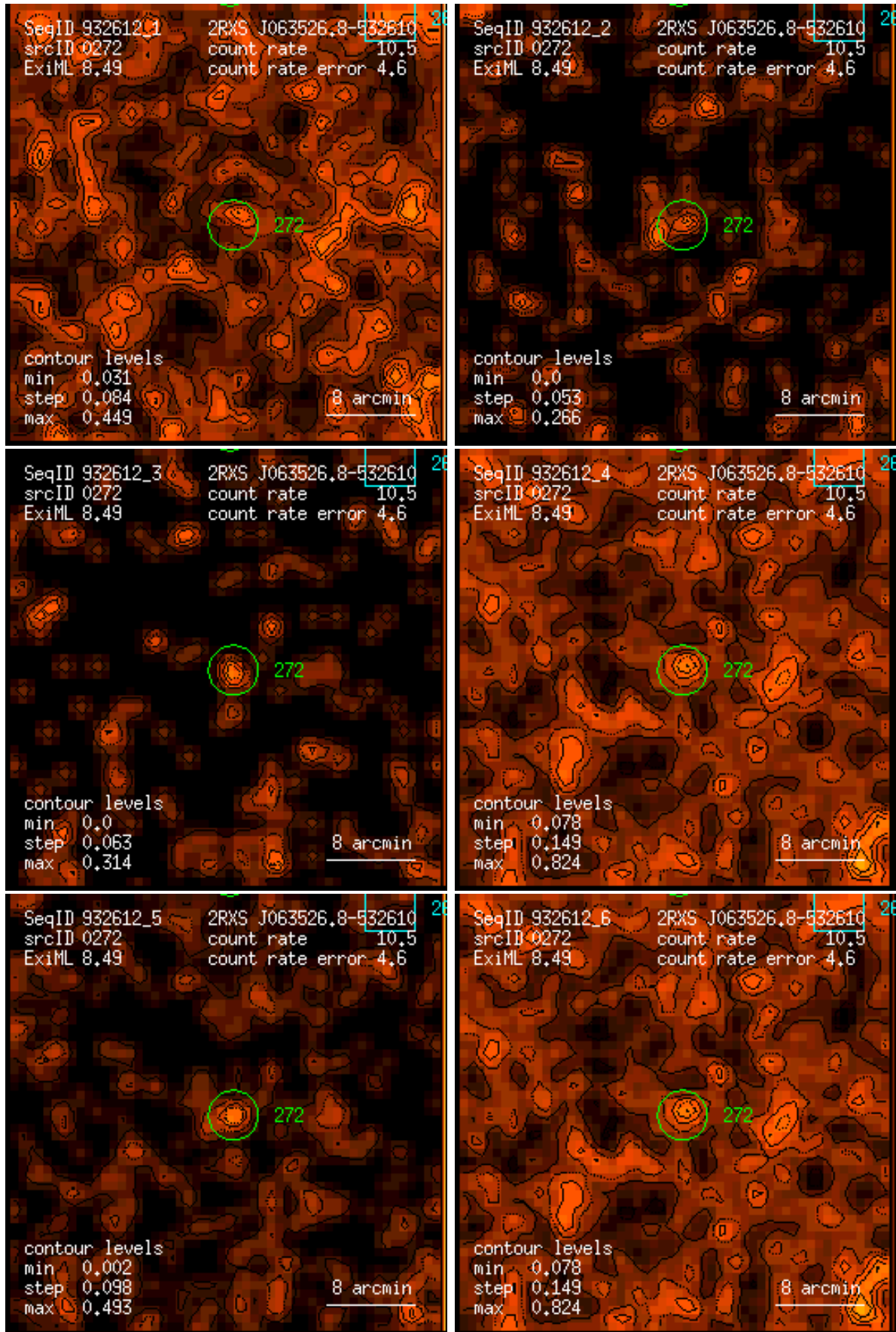
Figure 272: RASS 932612: detection 0272: band rate images, Gaussian filter: (1) PSPC channels 11 – 41, (2) 52 – 90, (3) 91 – 201, (4) 11 – 235, (5) 52 – 201, (6) 11 – 201. Broad band rates in counts/ks. Band rate contour levels in counts/ks/arcmin 2 .
