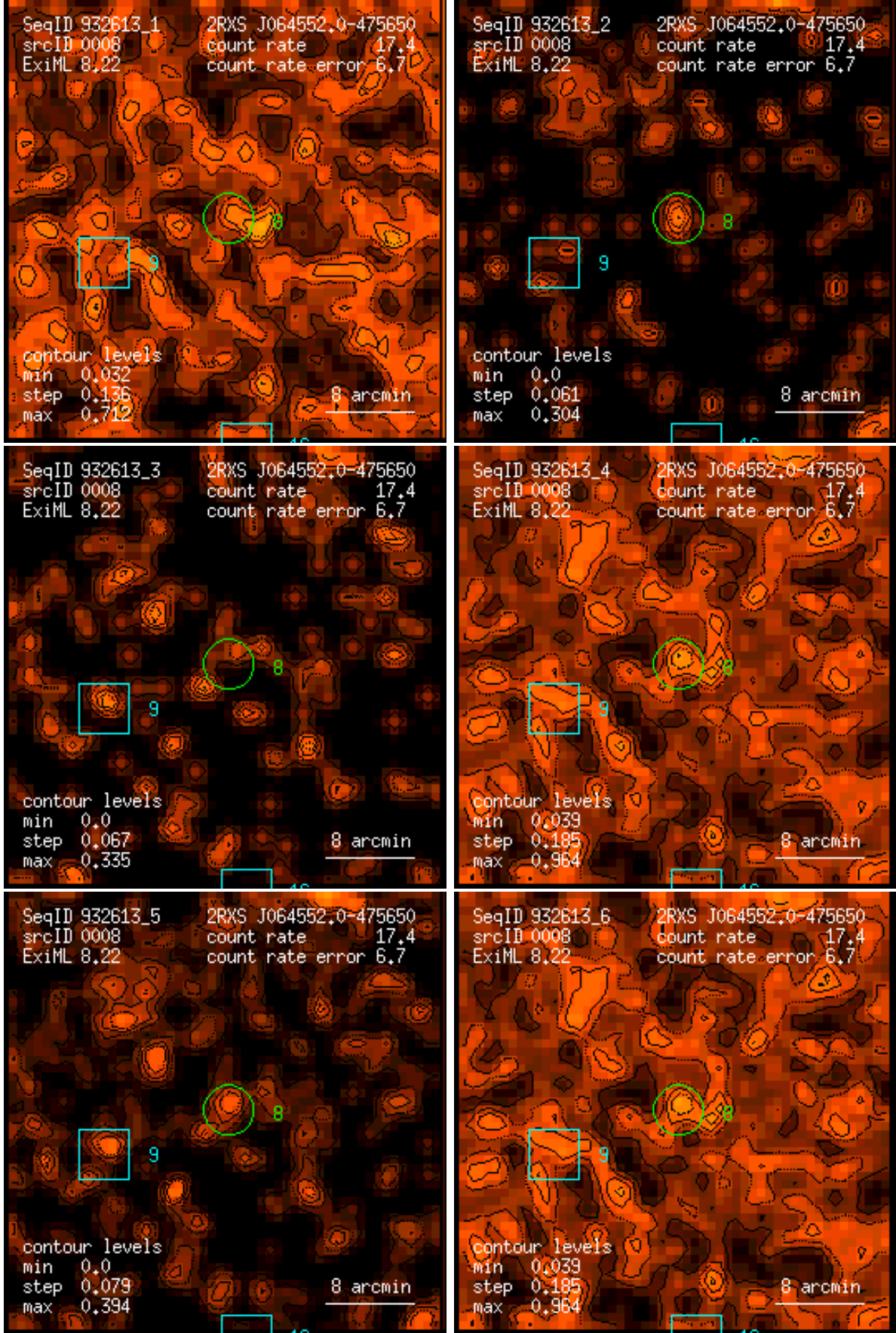
Figure 8: RASS 932613: detection 0008: band rate images, Gaussian filter: (1) PSPC channels 11 – 41, (2) 52 – 90, (3) 91 – 201, (4) 11 – 235, (5) 52 – 201, (6) 11 – 201. Broad band rates in counts/ks. Band rate contour levels in counts/ks/arcmin 2 .
