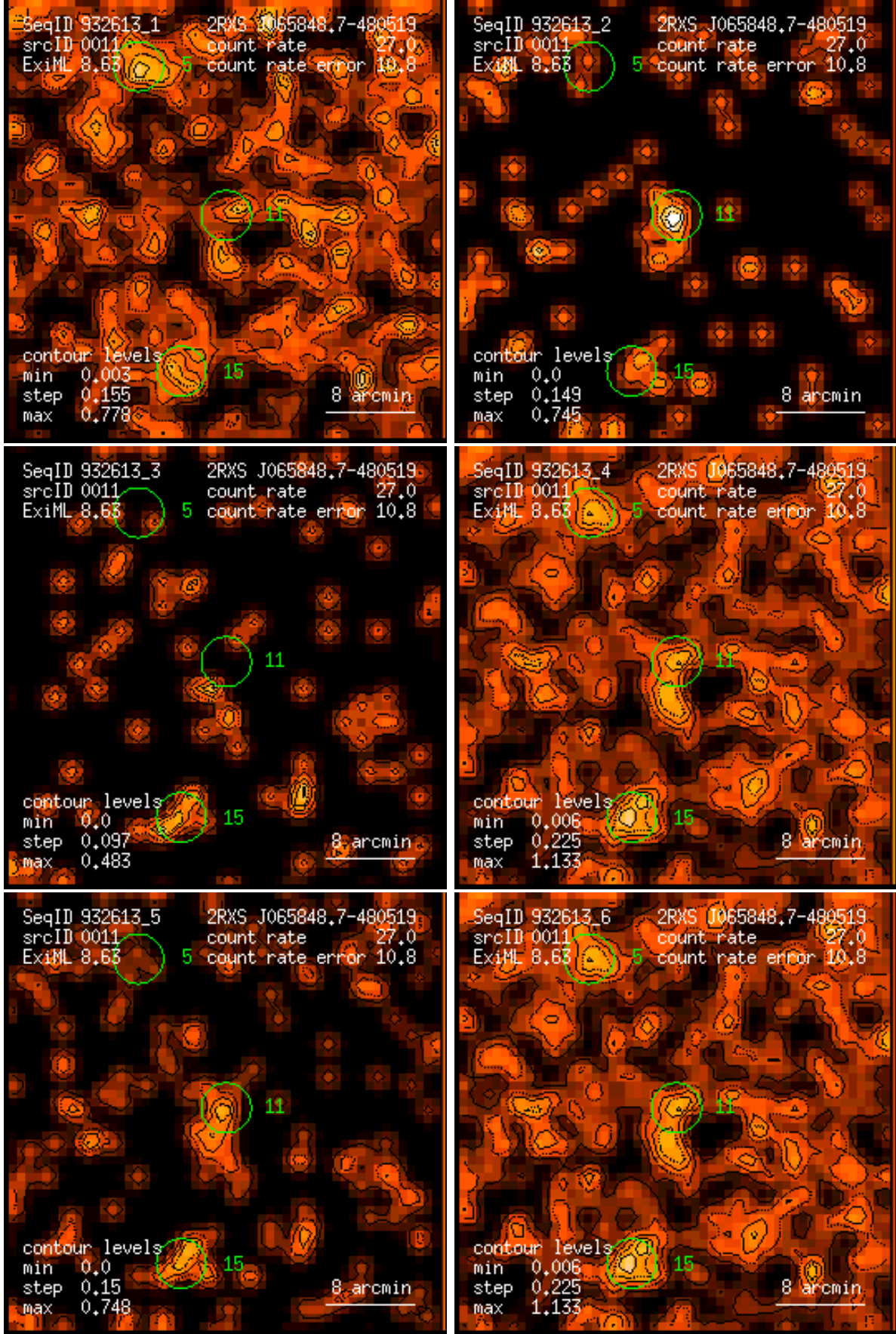
Figure 11: RASS 932613: detection 0011: band rate images, Gaussian filter: (1) PSPC channels 11 – 41, (2) 52 – 90, (3) 91 – 201, (4) 11 – 235, (5) 52 – 201, (6) 11 – 201. Broad band rates in counts/ks. Band rate contour levels in counts/ks/arcmin 2 .
