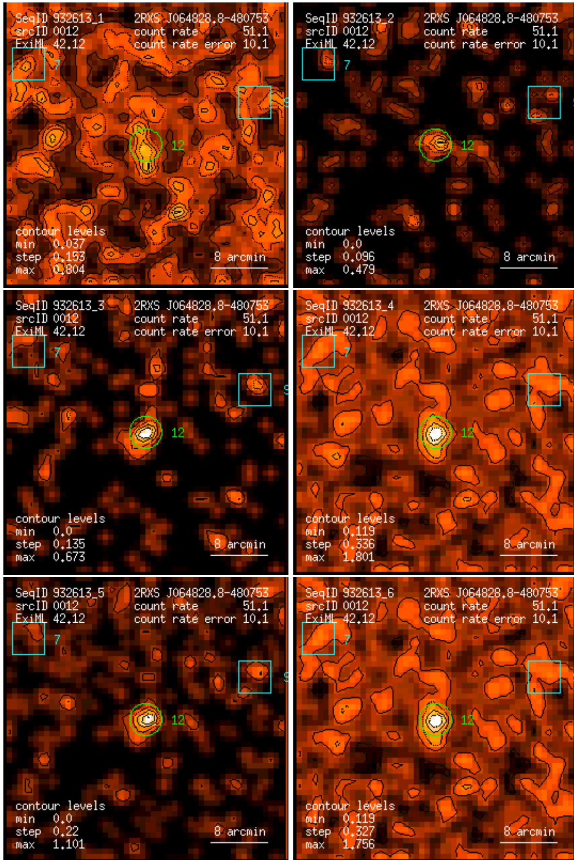
Figure 12: RASS 932613: detection 0012: band rate images, Gaussian filter: (1) PSPC channels 11 – 41, (2) 52 – 90, (3) 91 – 201, (4) 11 – 235, (5) 52 – 201, (6) 11 – 201. Broad band rates in counts/ks. Band rate contour levels in counts/ks/arcmin 2 .
