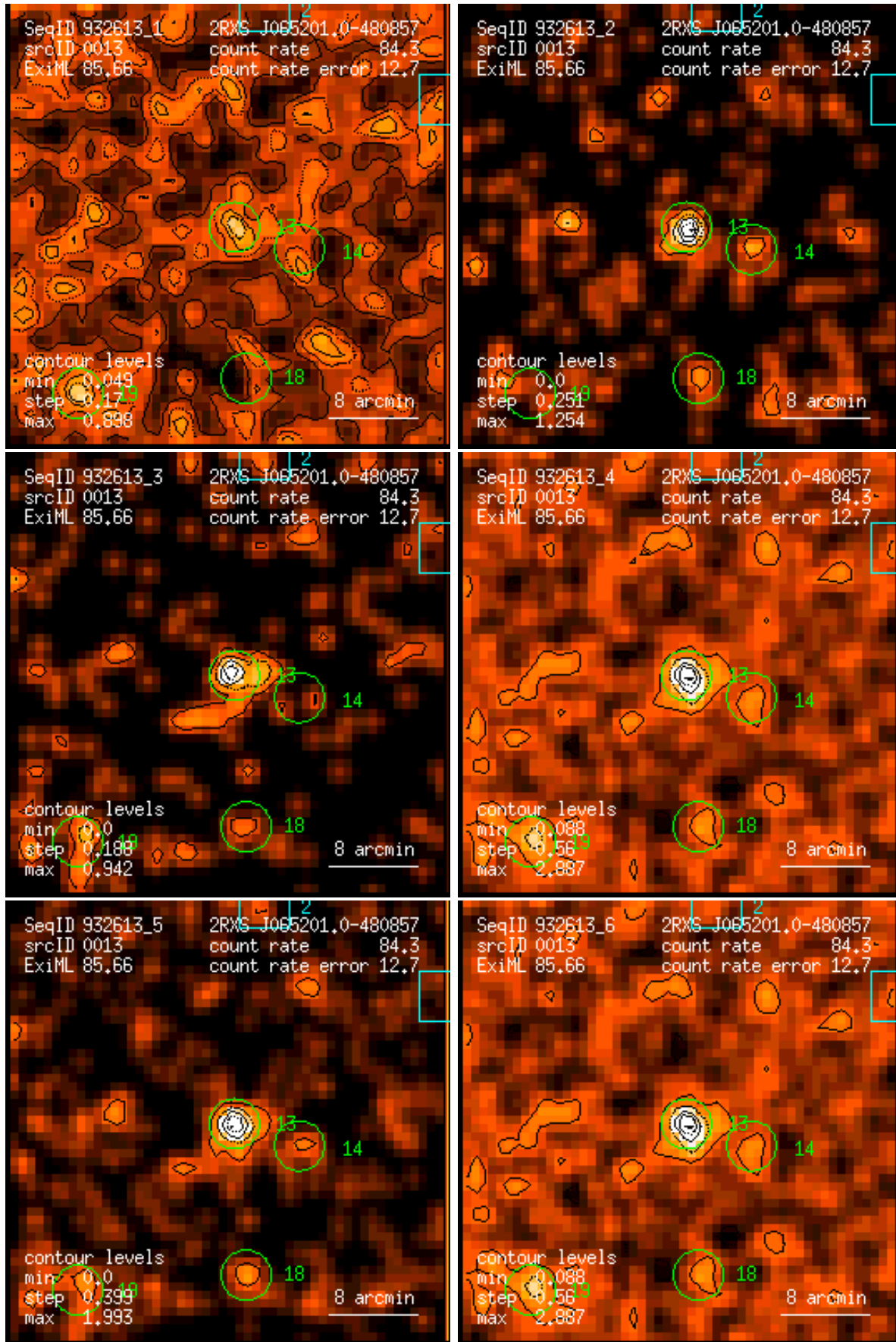
Figure 13: RASS 932613: detection 0013: band rate images, Gaussian filter: (1) PSPC channels 11 – 41, (2) 52 – 90, (3) 91 – 201, (4) 11 – 235, (5) 52 – 201, (6) 11 – 201. Broad band rates in counts/ks. Band rate contour levels in counts/ks/arcmin 2 .
