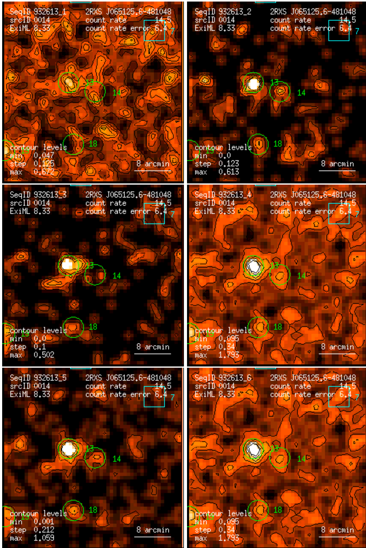
Figure 14: RASS 932613: detection 0014: band rate images, Gaussian filter: (1) PSPC channels 11 – 41, (2) 52 – 90, (3) 91 – 201, (4) 11 – 235, (5) 52 – 201, (6) 11 – 201. Broad band rates in counts/ks. Band rate contour levels in counts/ks/arcmin 2 .
