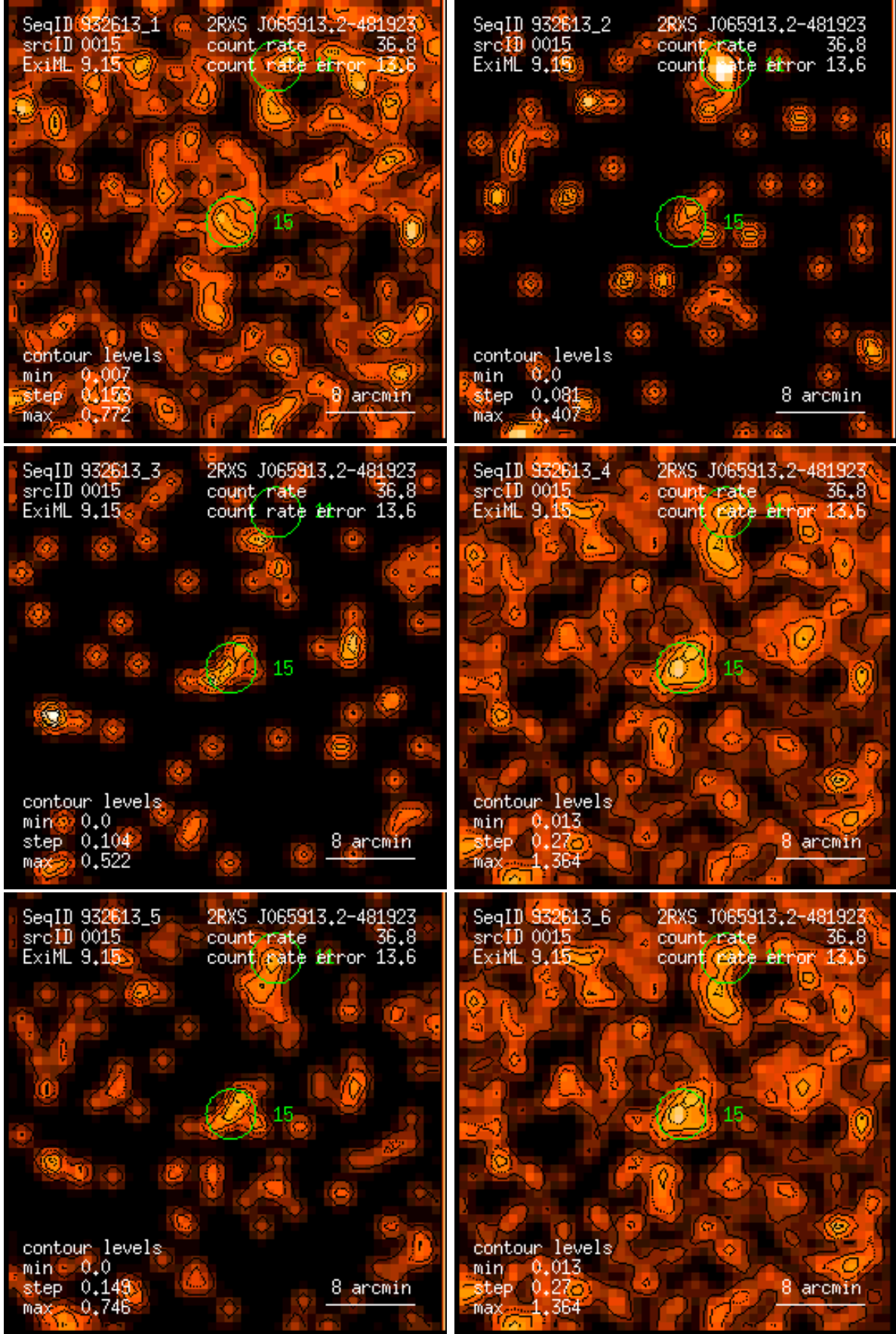
Figure 15: RASS 932613: detection 0015: band rate images, Gaussian filter: (1) PSPC channels 11 – 41, (2) 52 – 90, (3) 91 – 201, (4) 11 – 235, (5) 52 – 201, (6) 11 – 201. Broad band rates in counts/ks. Band rate contour levels in counts/ks/arcmin 2 .
