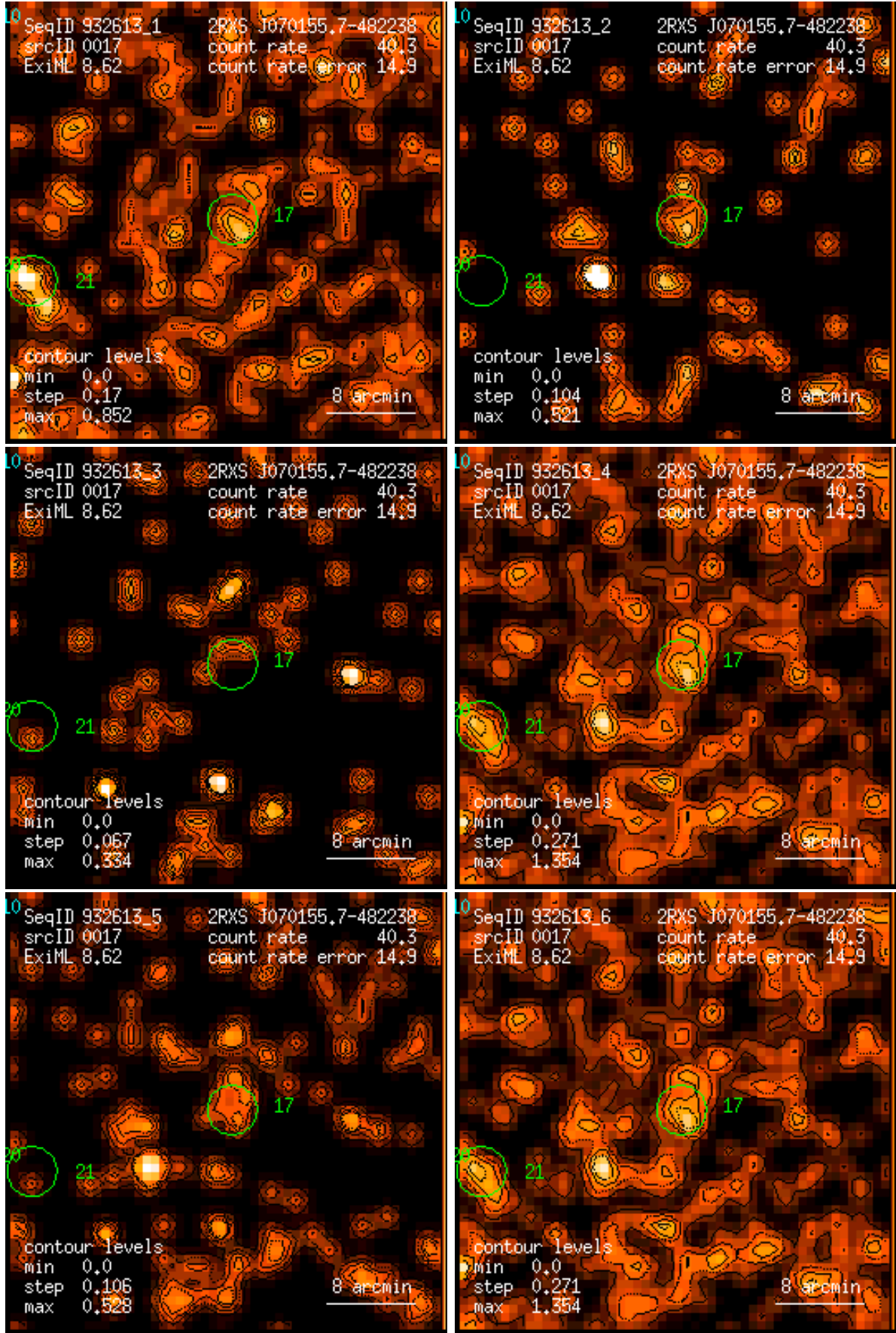
Figure 17: RASS 932613: detection 0017: band rate images, Gaussian filter: (1) PSPC channels 11 – 41, (2) 52 – 90, (3) 91 – 201, (4) 11 – 235, (5) 52 – 201, (6) 11 – 201. Broad band rates in counts/ks. Band rate contour levels in counts/ks/arcmin 2 .
