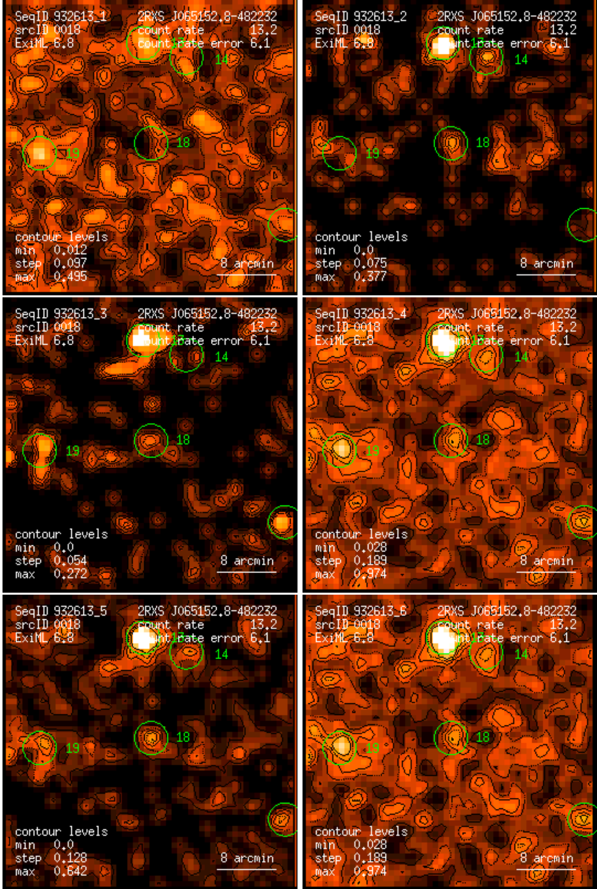
Figure 18: RASS 932613: detection 0018: band rate images, Gaussian filter: (1) PSPC channels 11 – 41, (2) 52 – 90, (3) 91 – 201, (4) 11 – 235, (5) 52 – 201, (6) 11 – 201. Broad band rates in counts/ks. Band rate contour levels in counts/ks/arcmin 2 .
