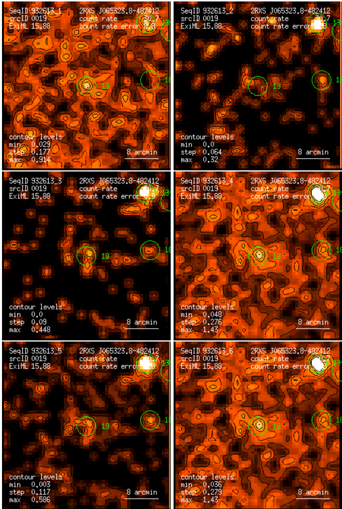
Figure 19: RASS 932613: detection 0019: band rate images, Gaussian filter: (1) PSPC channels 11 – 41, (2) 52 – 90, (3) 91 – 201, (4) 11 – 235, (5) 52 – 201, (6) 11 – 201. Broad band rates in counts/ks. Band rate contour levels in counts/ks/arcmin 2 .
