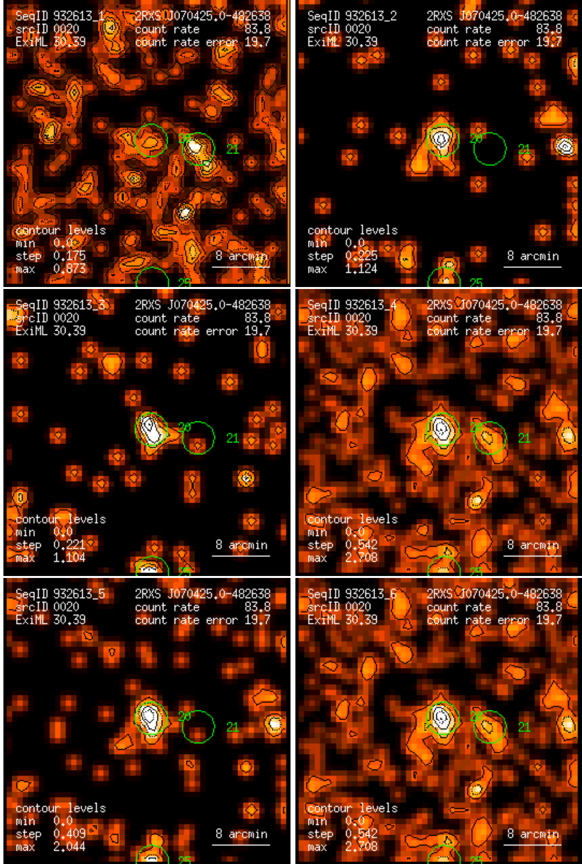
Figure 20: RASS 932613: detection 0020: band rate images, Gaussian filter: (1) PSPC channels 11 – 41, (2) 52 – 90, (3) 91 – 201, (4) 11 – 235, (5) 52 – 201, (6) 11 – 201. Broad band rates in counts/ks. Band rate contour levels in counts/ks/arcmin 2 .
