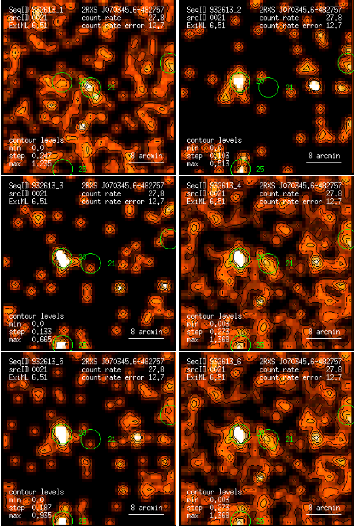
Figure 21: RASS 932613: detection 0021: band rate images, Gaussian filter: (1) PSPC channels 11 – 41, (2) 52 – 90, (3) 91 – 201, (4) 11 – 235, (5) 52 – 201, (6) 11 – 201. Broad band rates in counts/ks. Band rate contour levels in counts/ks/arcmin 2 .
