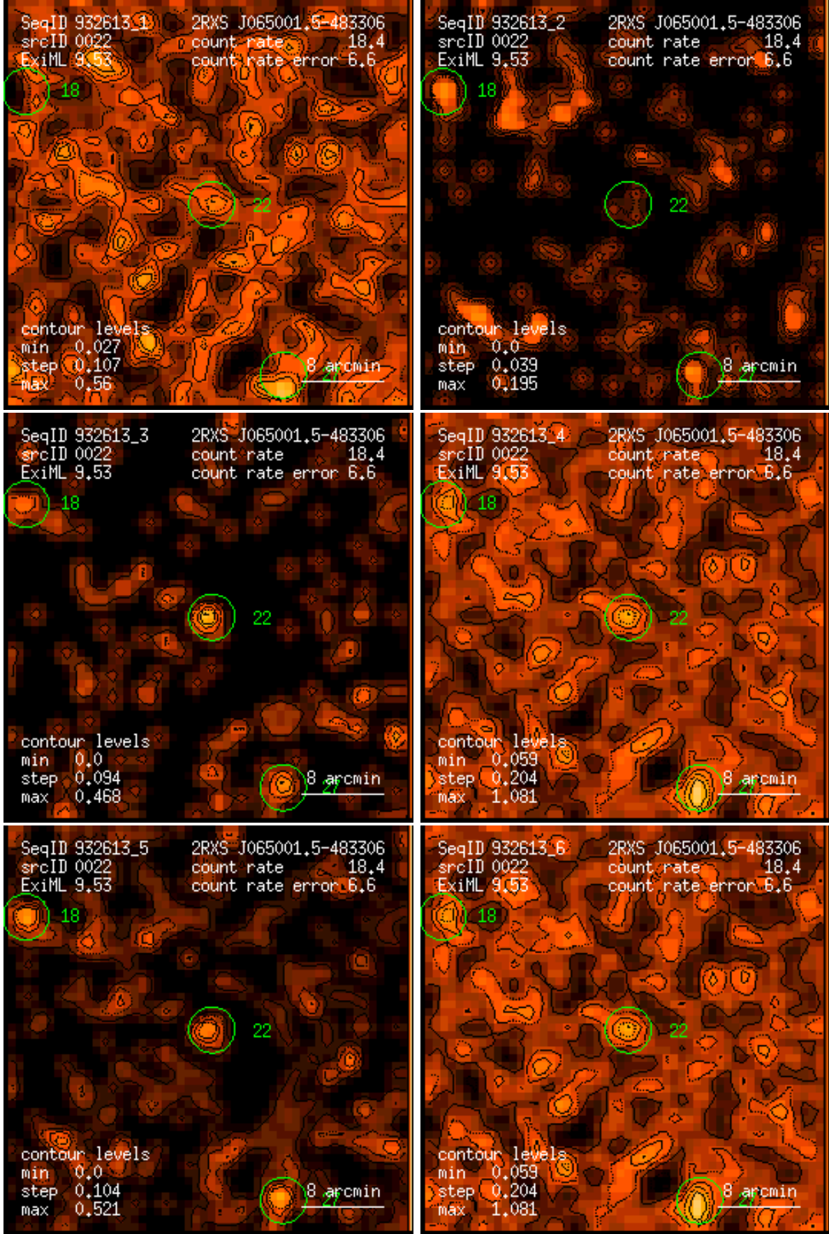
Figure 22: RASS 932613: detection 0022: band rate images, Gaussian filter: (1) PSPC channels 11 – 41, (2) 52 – 90, (3) 91 – 201, (4) 11 – 235, (5) 52 – 201, (6) 11 – 201. Broad band rates in counts/ks. Band rate contour levels in counts/ks/arcmin 2 .
