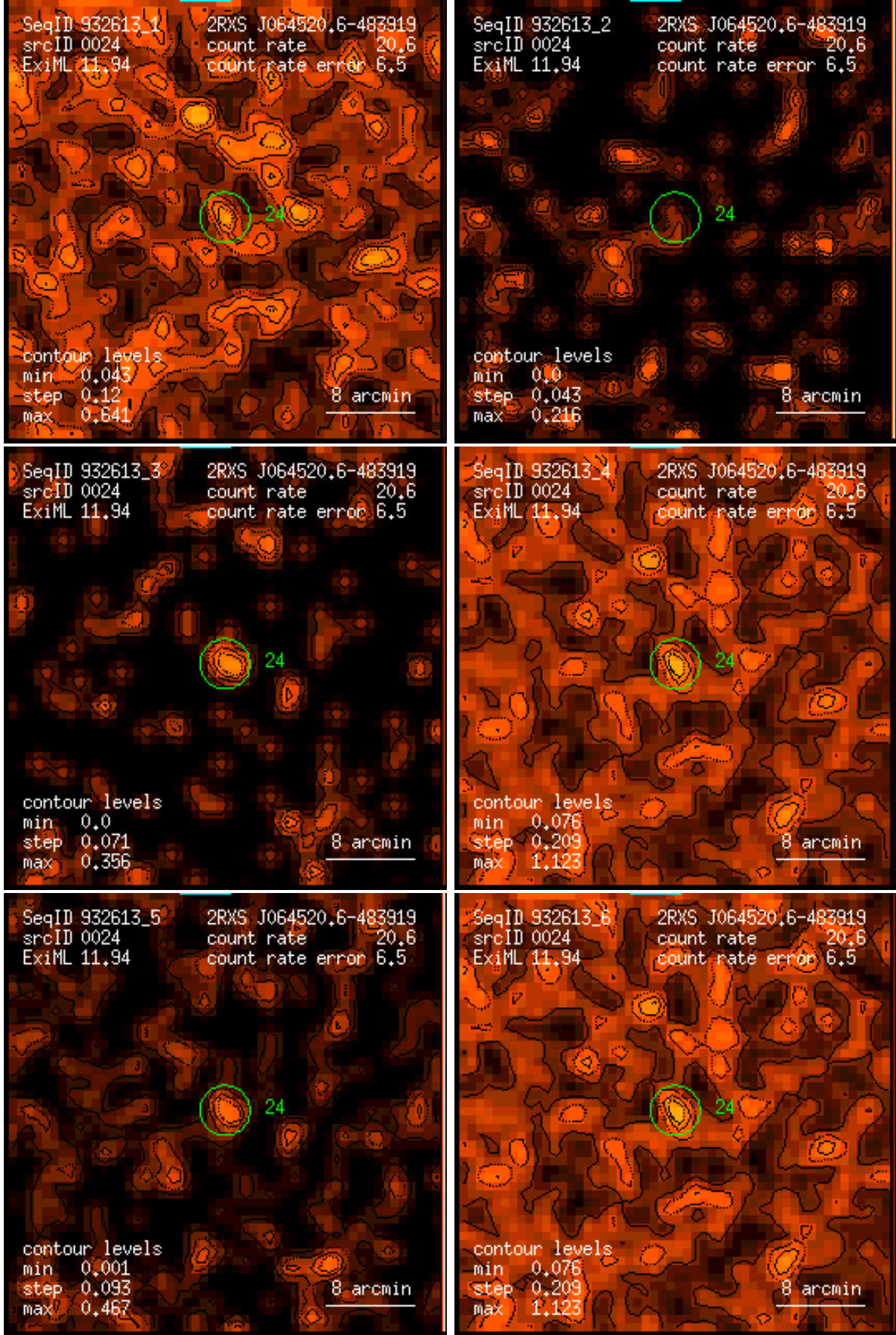
Figure 24: RASS 932613: detection 0024: band rate images, Gaussian filter: (1) PSPC channels 11 – 41, (2) 52 – 90, (3) 91 – 201, (4) 11 – 235, (5) 52 – 201, (6) 11 – 201. Broad band rates in counts/ks. Band rate contour levels in counts/ks/arcmin 2 .
