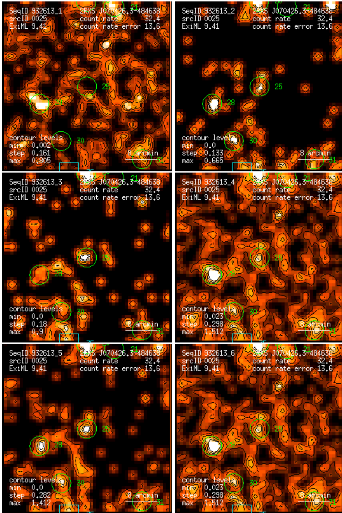
Figure 25: RASS 932613: detection 0025: band rate images, Gaussian filter: (1) PSPC channels 11 – 41, (2) 52 – 90, (3) 91 – 201, (4) 11 – 235, (5) 52 – 201, (6) 11 – 201. Broad band rates in counts/ks. Band rate contour levels in counts/ks/arcmin 2 .
